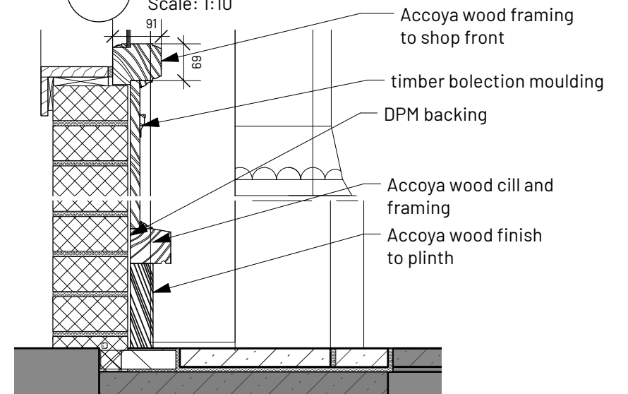
5 Proposed Shop Front Detail C Scale: 1:10
