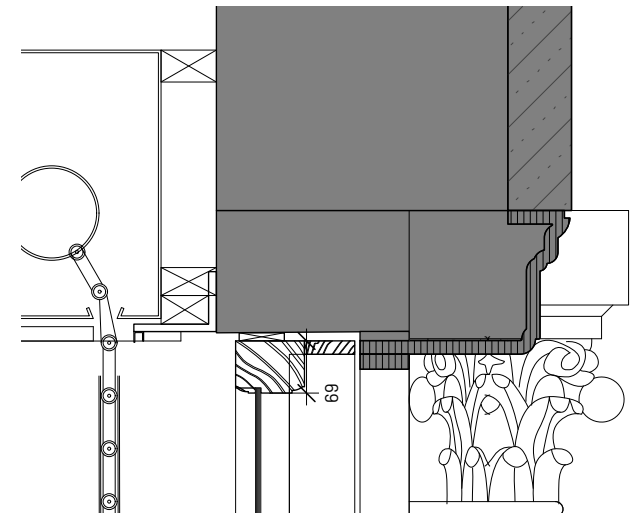
4 Proposed Shop Front Detail B Scale: 1:10
