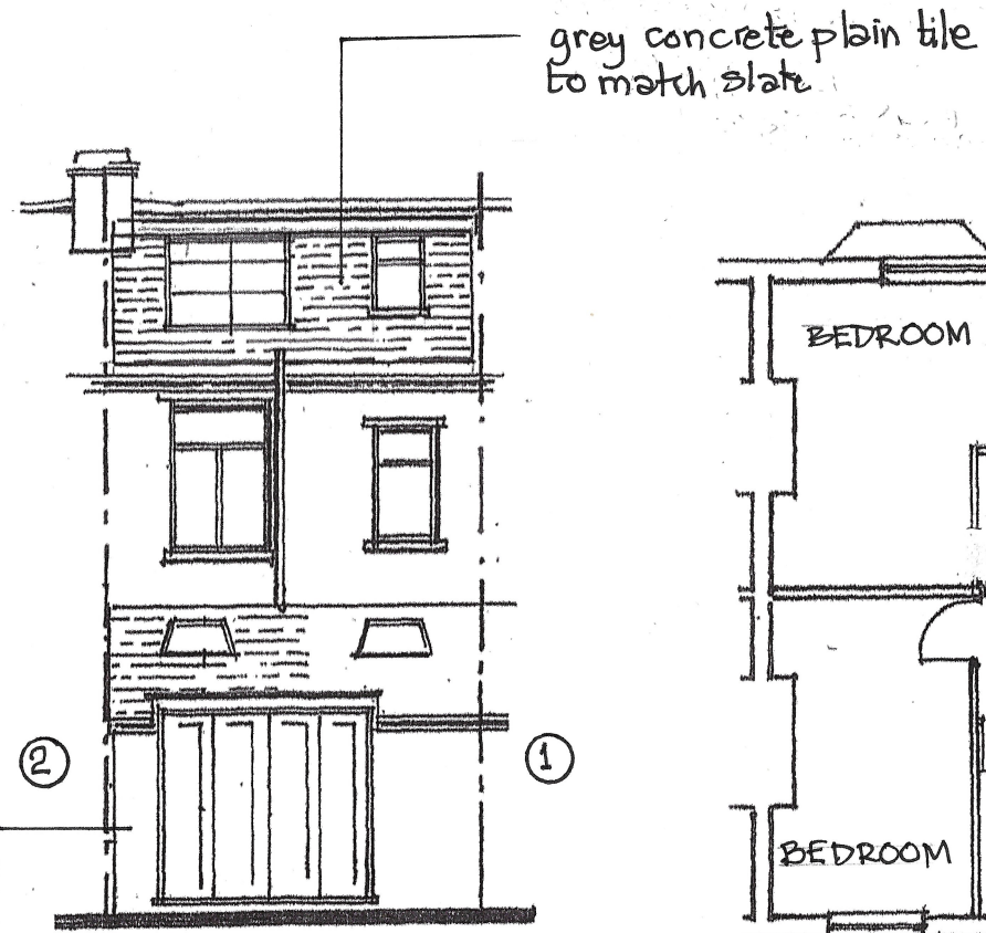
REAR ELEVATION
