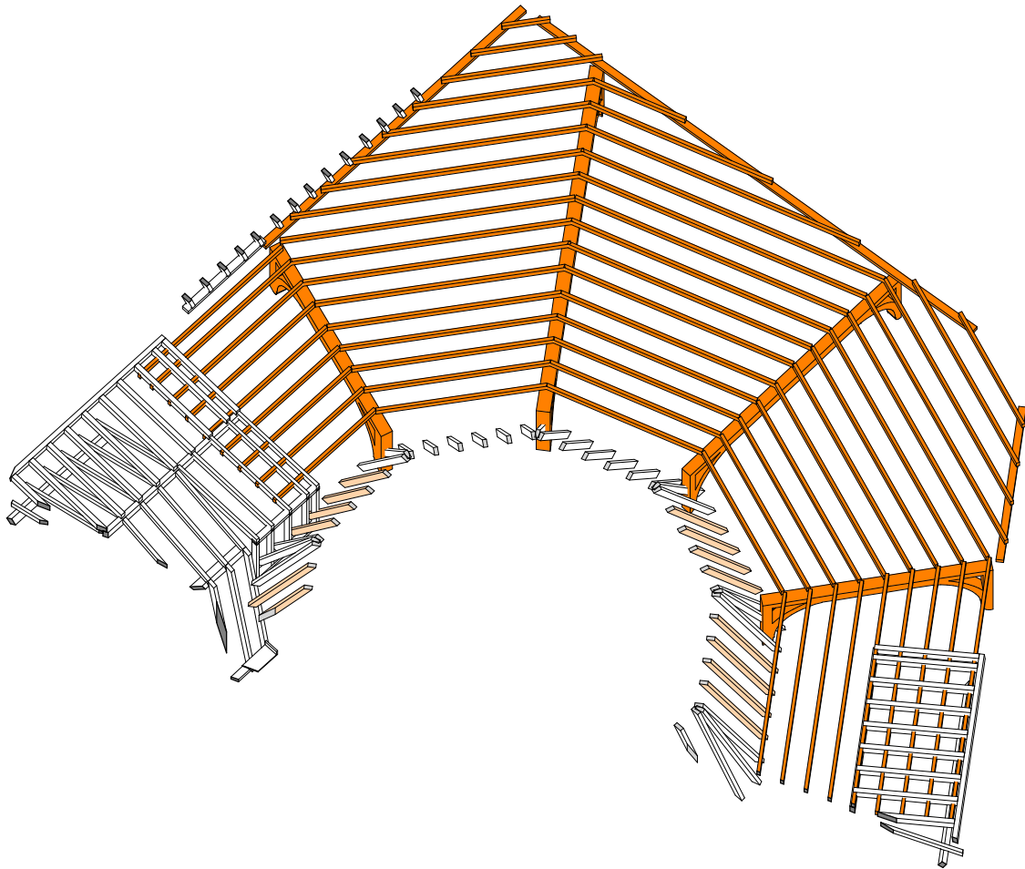
9b 3D View Area 9 - Structure Only
