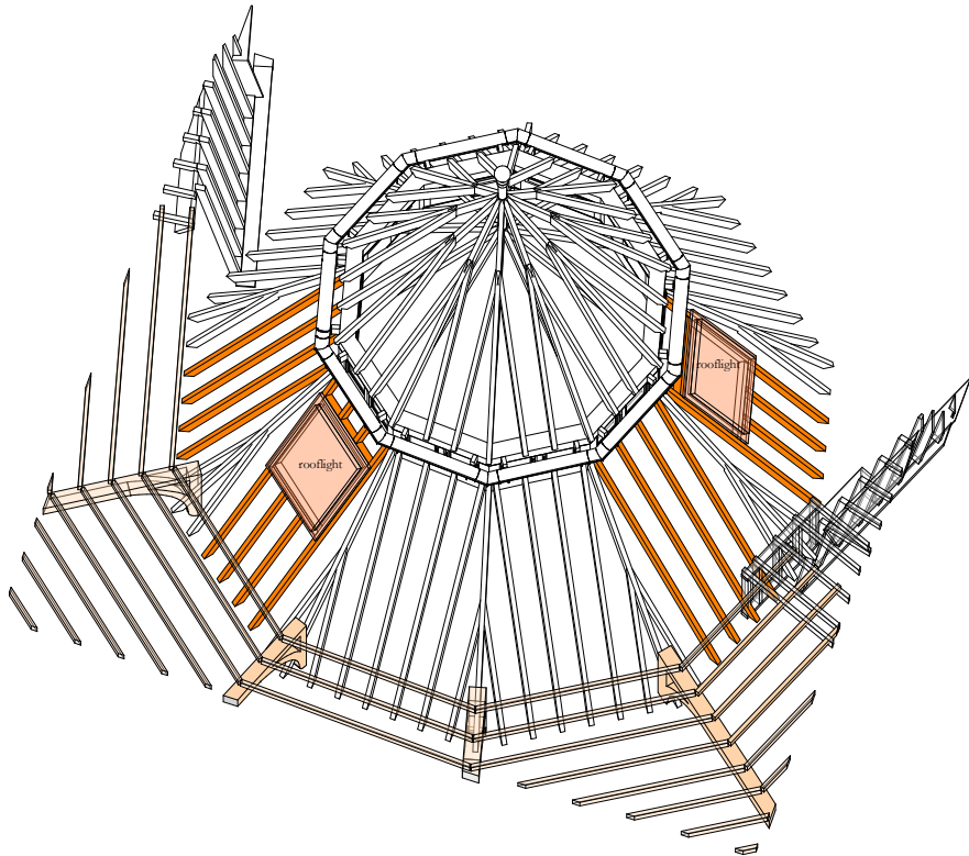
10b 3D View Area 10 - Structure Only
