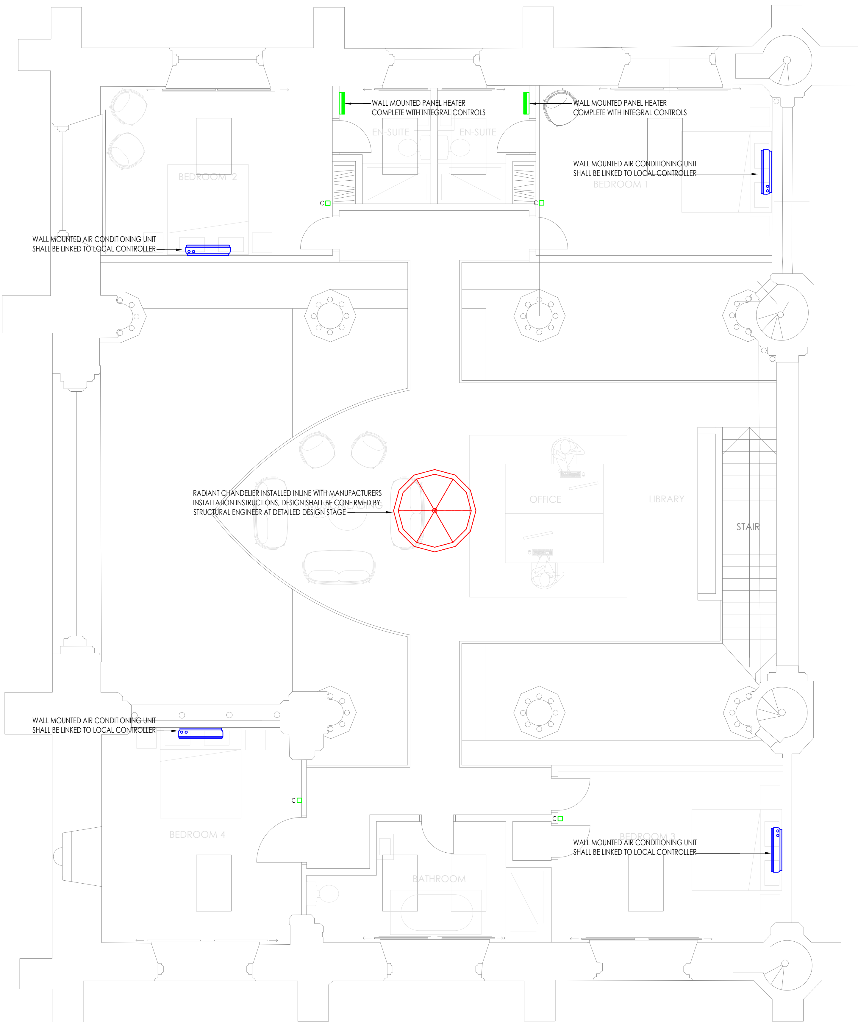
INDICATIVE HEATING STRATEGY, FIRST FLOOR SCALE 1:50 @A0
