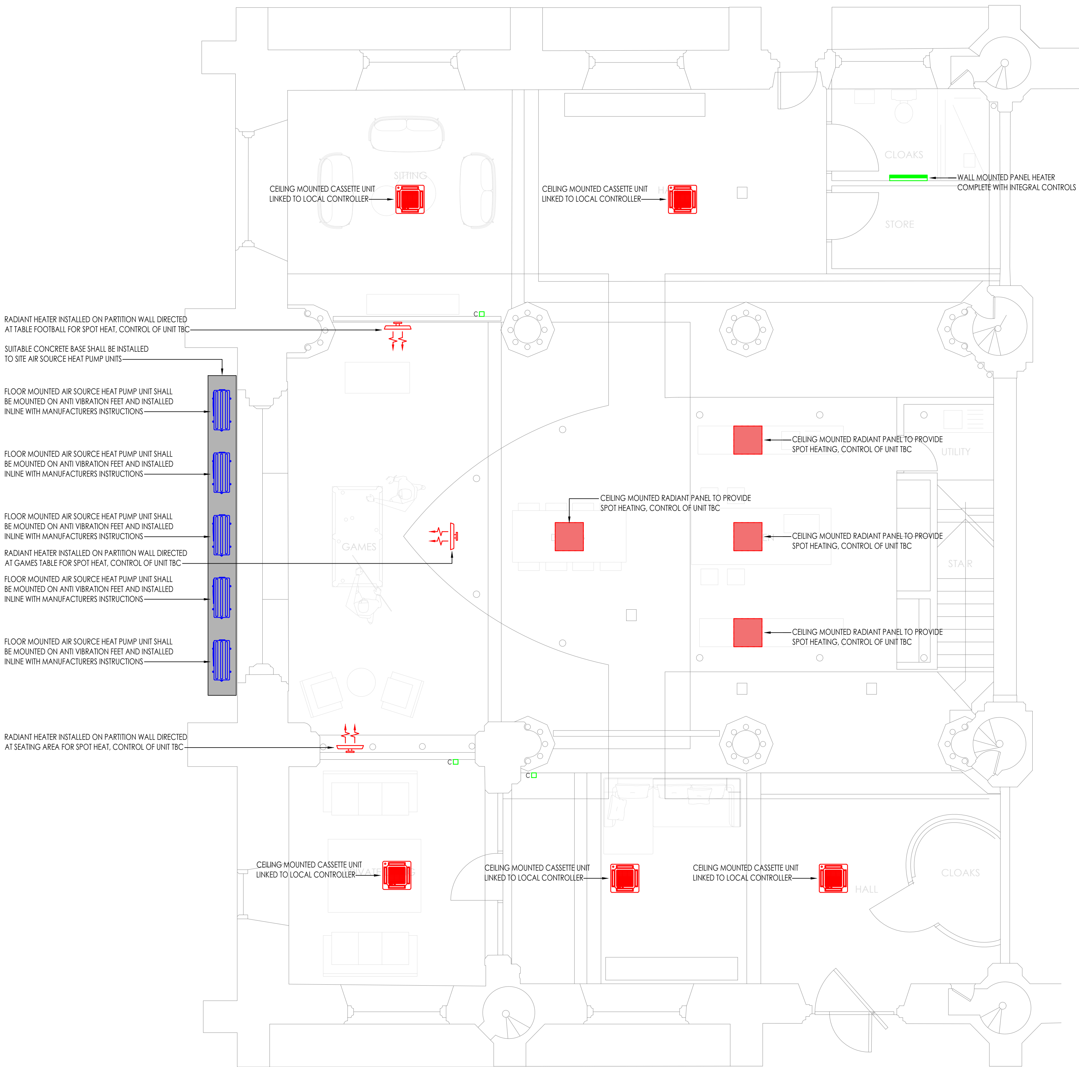
INDICATIVE HEATING STRATEGY, GROUND FLOOR SCALE 1:50 @A0
