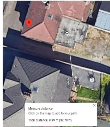
Figure 8 Distance from the middle of the flat roof to the nearest habitable window
