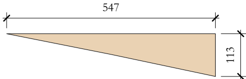
TcR_23 Elevation Front 1 : 10
