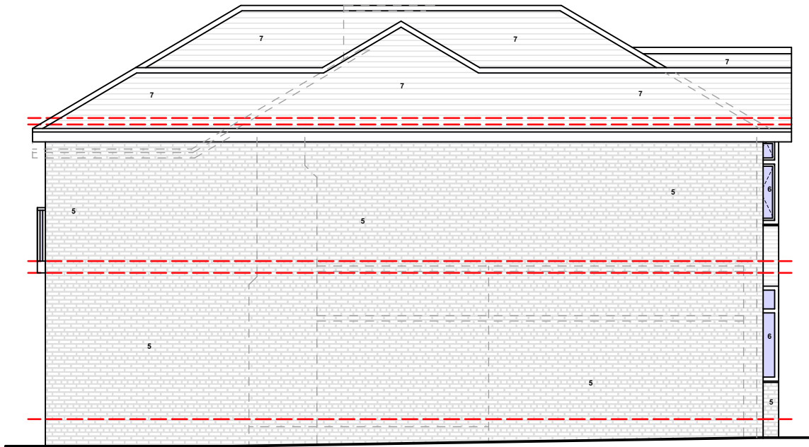
PROPOSED GA SIDE ELEVATION 1
