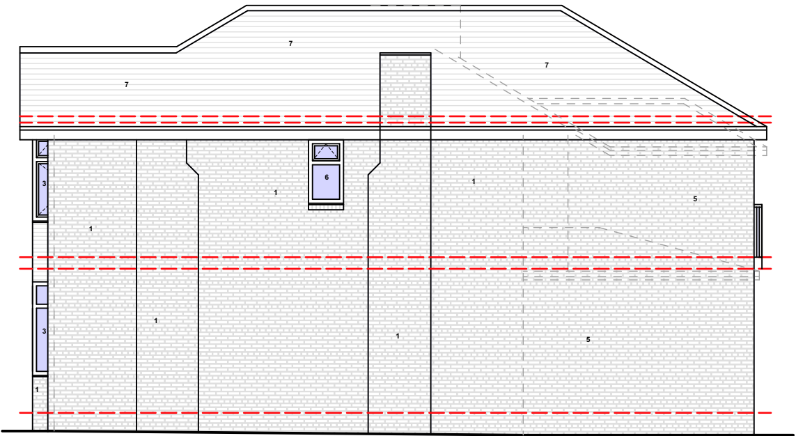
PROPOSED GA SIDE ELEVATION 2
