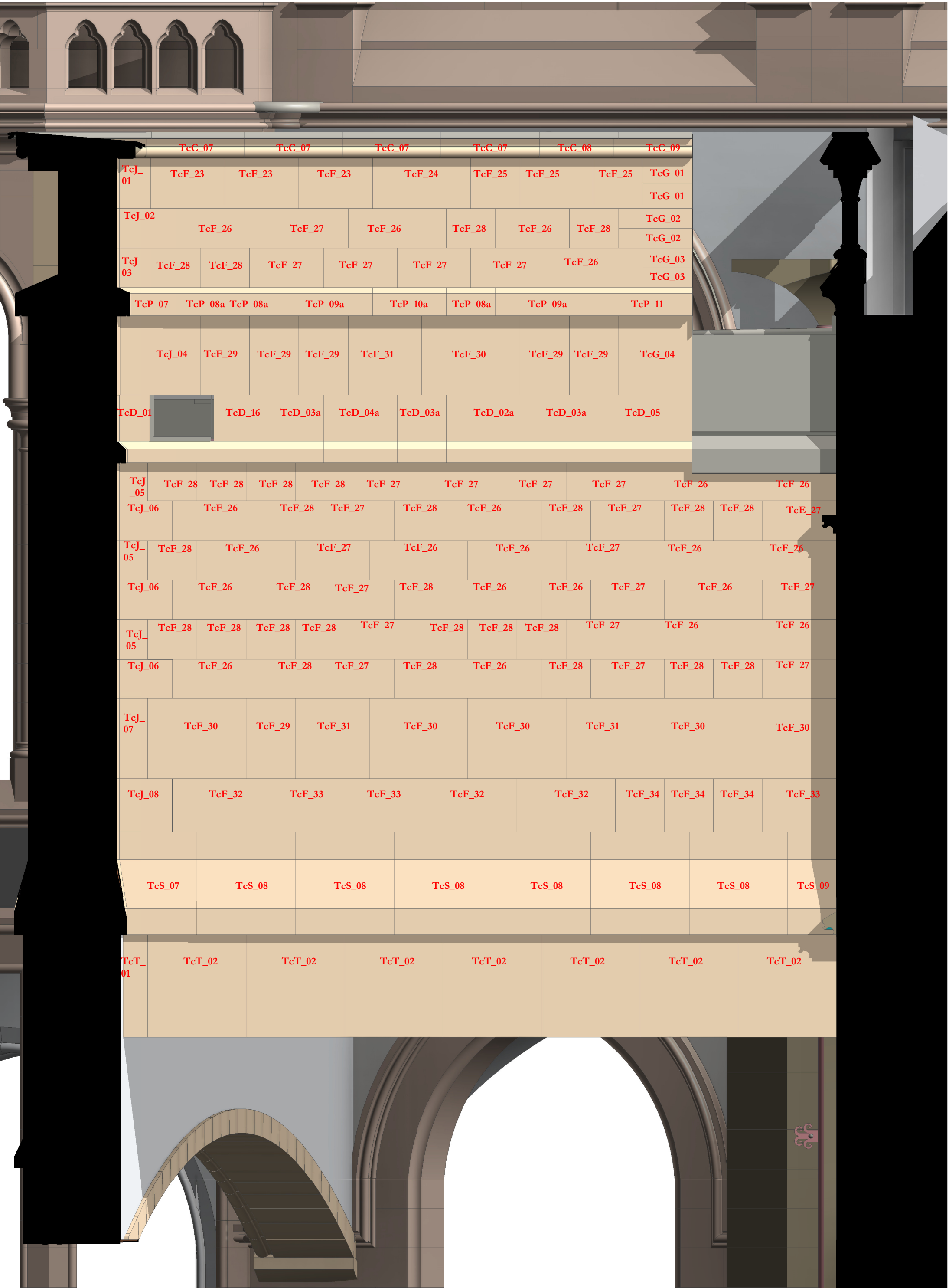
South Terracotta Elevation 02 1 : 20
