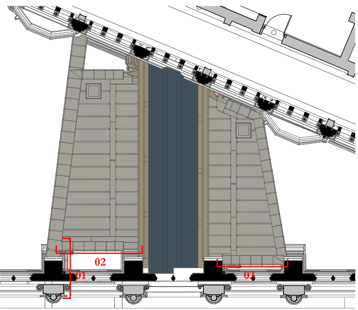
Link Bridge Terracotta Key Plan - South 1 : 200
