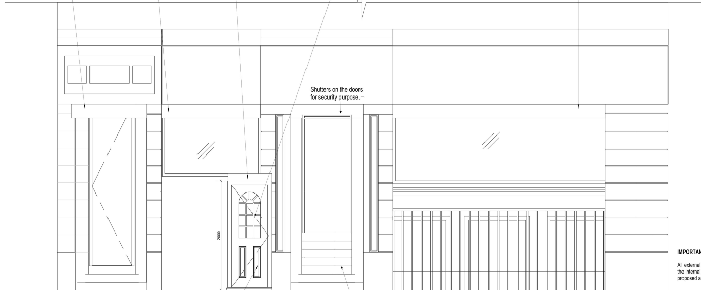
Proposed Front Elevation 1 : 25
