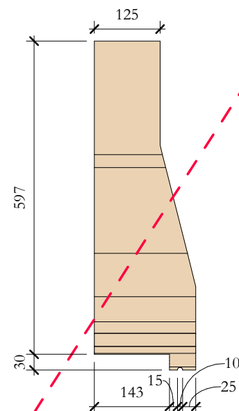
TcS_12 Elevation Left
