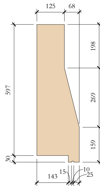
TcS_13 Elevation Left
