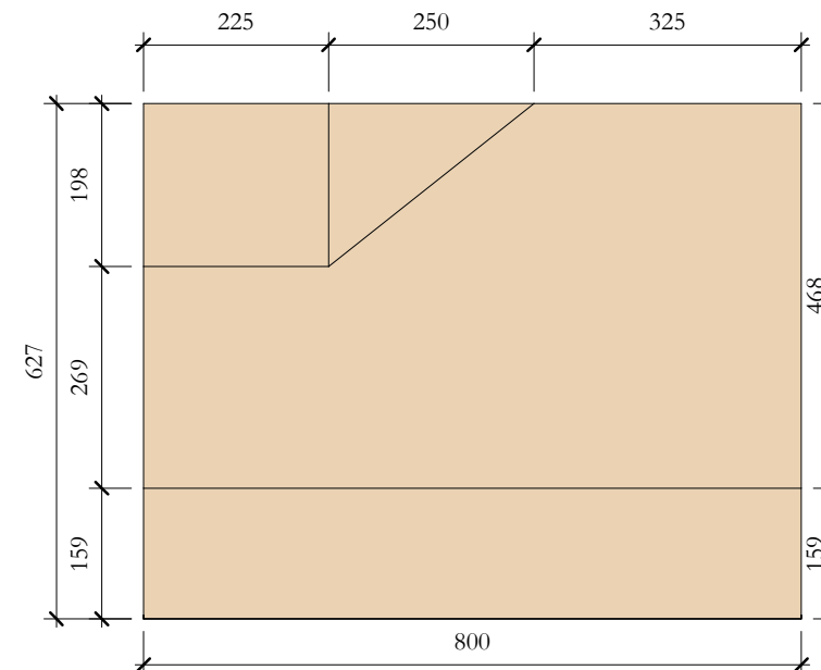
TcS_13 Elevation Front
