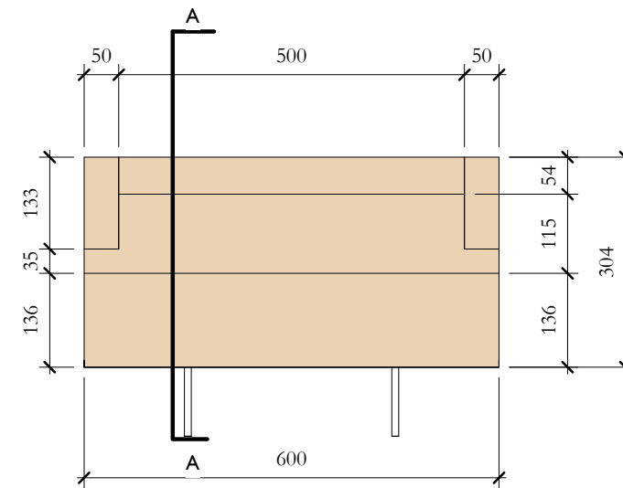
TcP_05 Elevation Front 1 : 10
