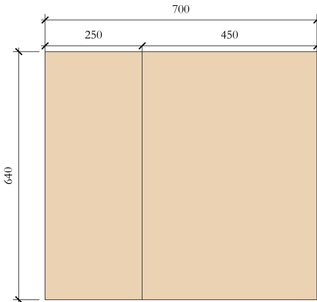
TcW_08 Elevation Front 1 : 10
