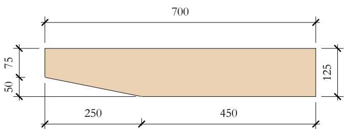
TcW_08 Elevation Top 1 : 10
