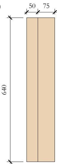
TcW_07 Elevation Right 1 : 10
