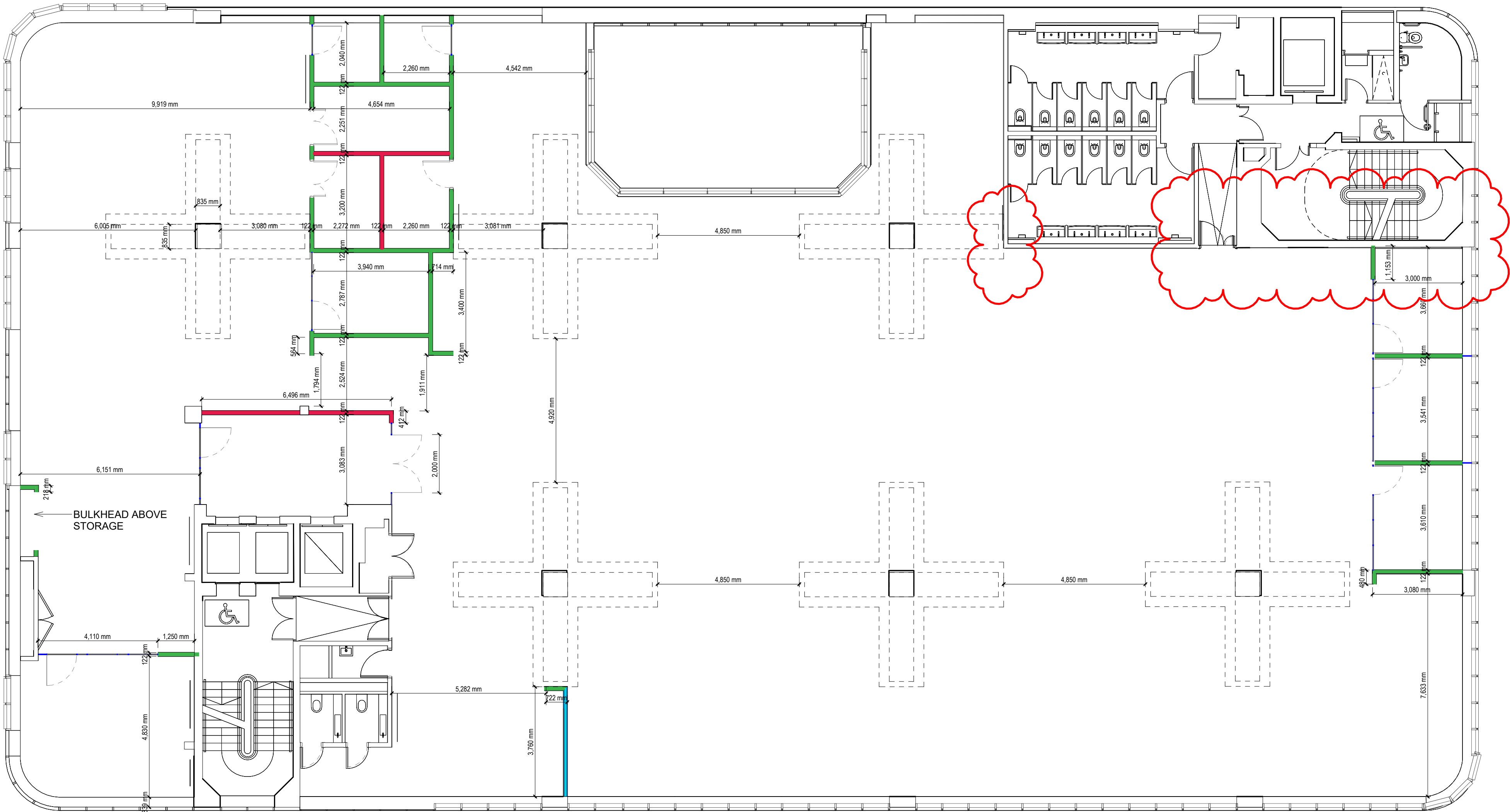
Setting out Plan - Level 03
