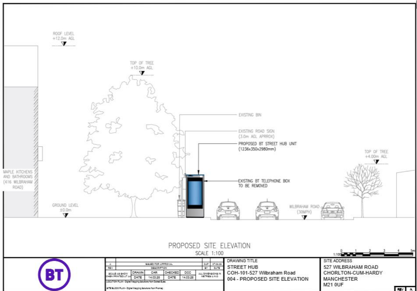
Submitted proposed site elevation
