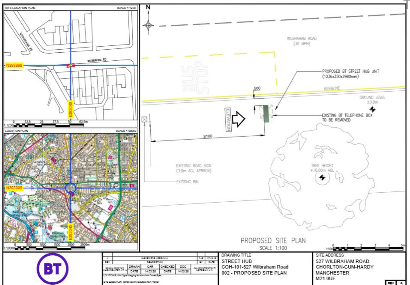
Submitted proposed site plan
