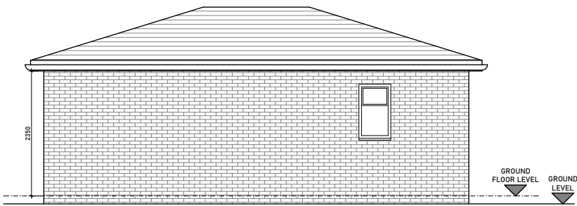
REAR ELEVATION 1:100
