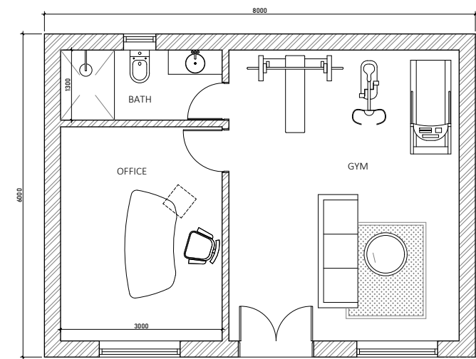
FLOOR PLAN 1:100
