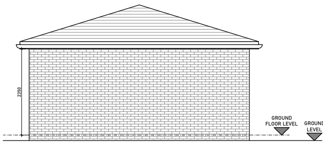
LEFT ELEVATION 1:100
