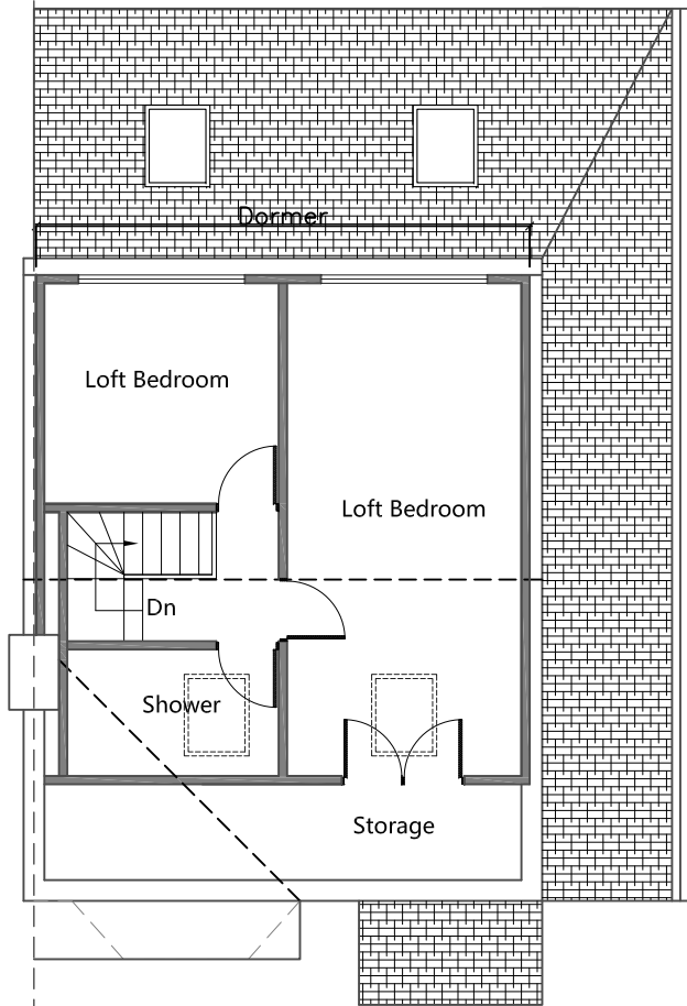
Proposed Loft Floor Plan
