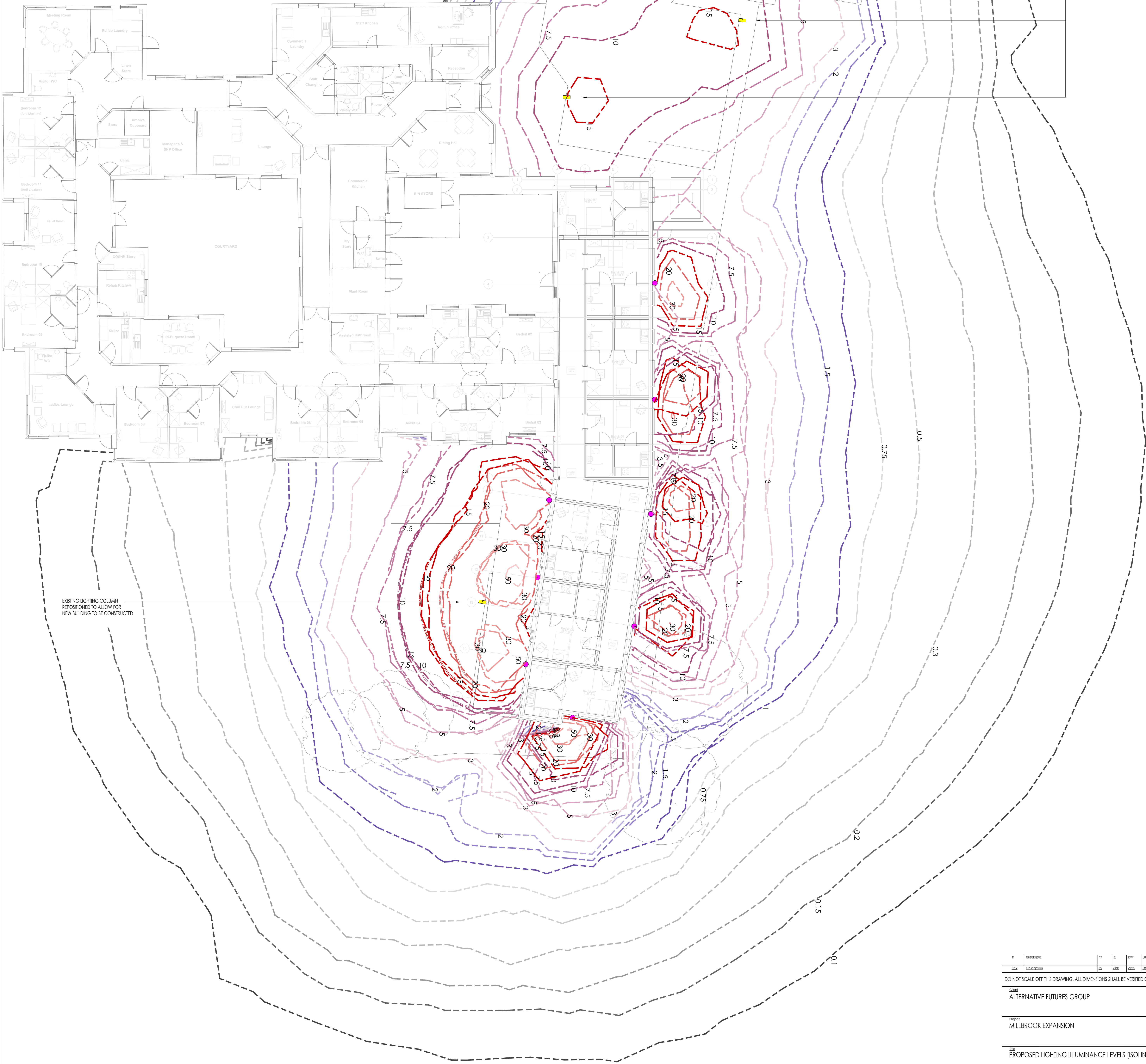
PROPOSED LIGHTING ILLUMINANCE LEVELS (ISOLINES) SCALE 1:100 @ A0
