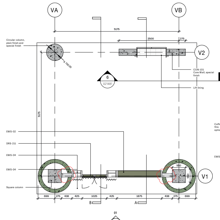
02 VMU - GROUND FLOOR PLAN 021481 1:50
