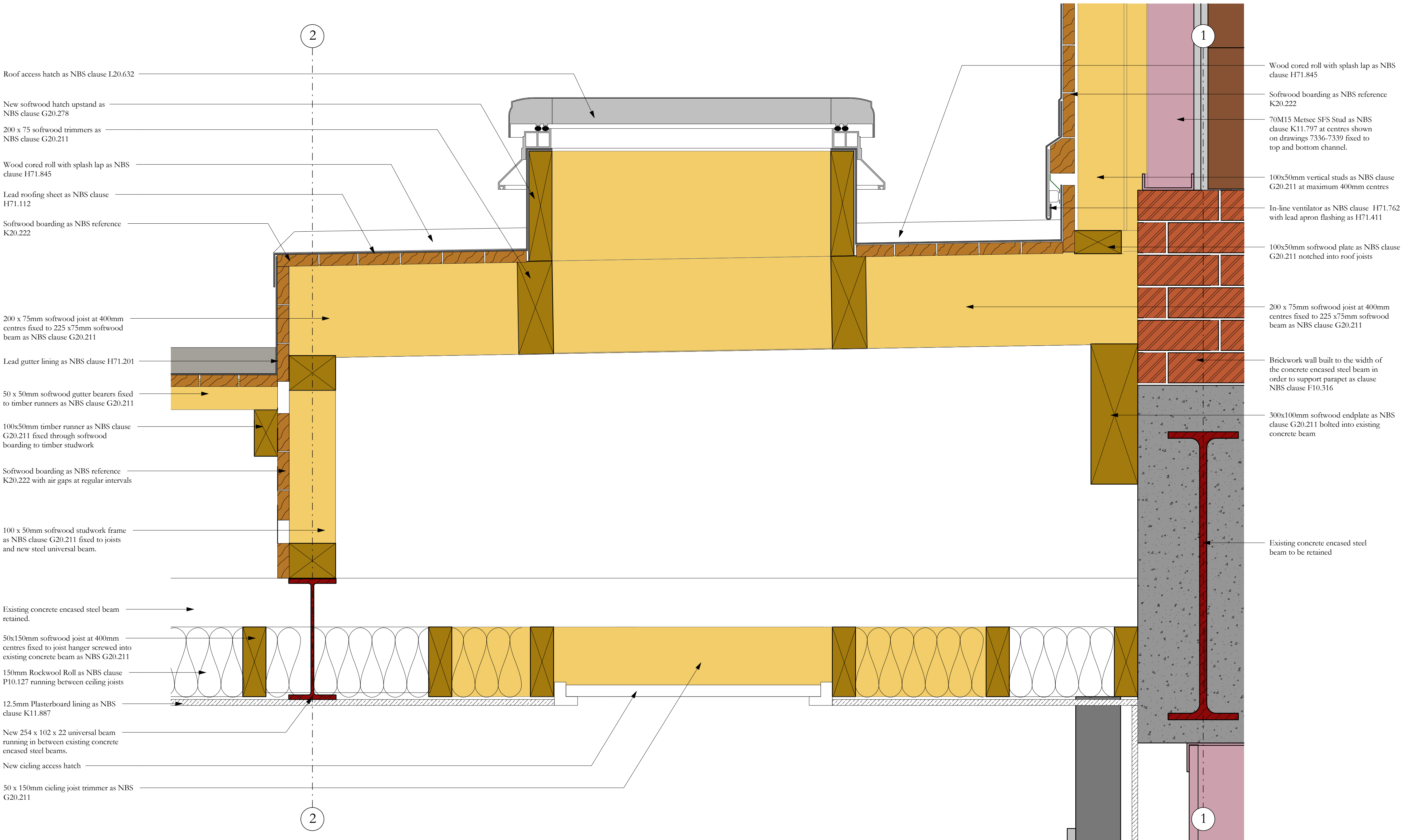
Roof access Hatch detail 1:5
