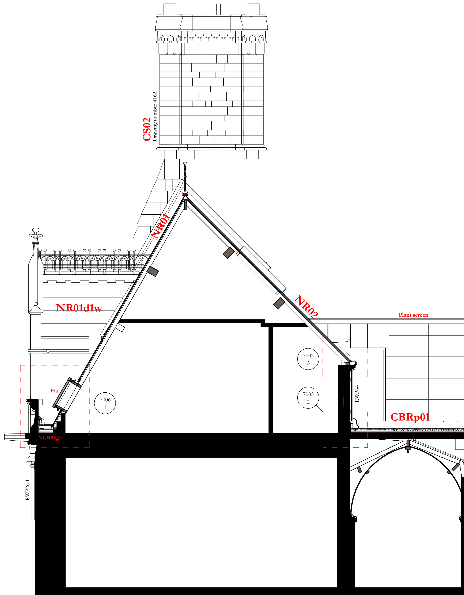
Section AA
