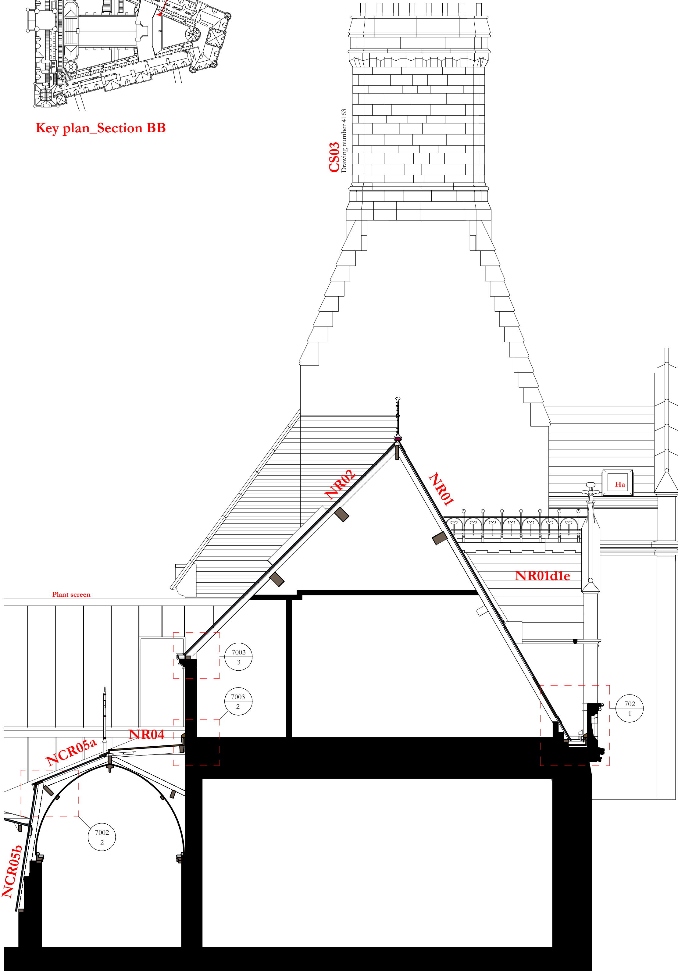
Section BB
