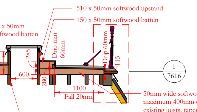
Section J-J
