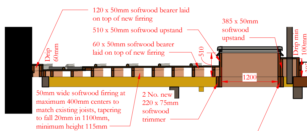
Section C-C
