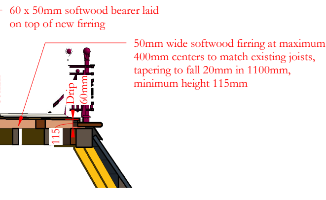
Section H-H
