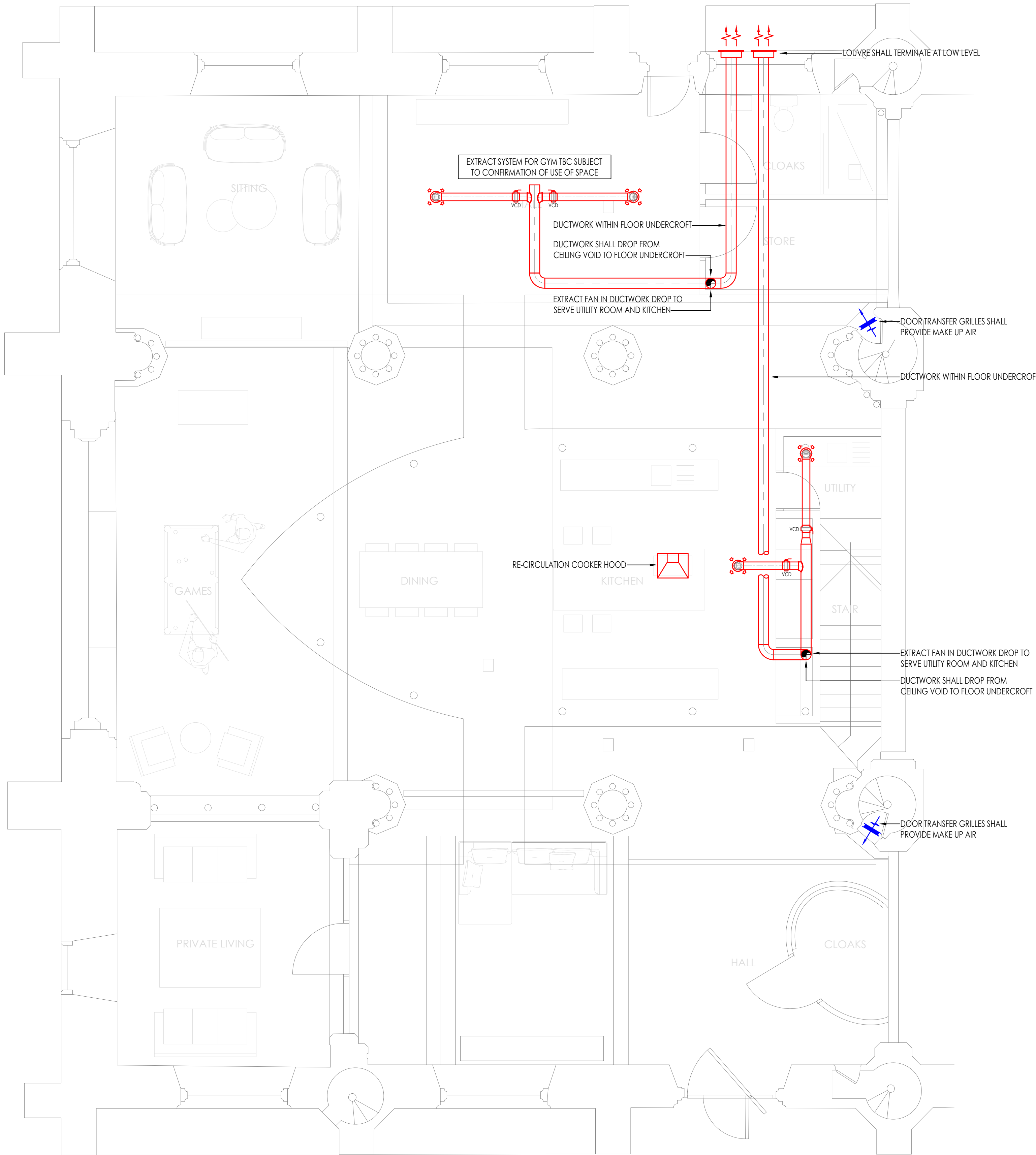
INDICATIVE VENTILATION STRATEGY, GROUND FLOOR SCALE 1:50 @A0
