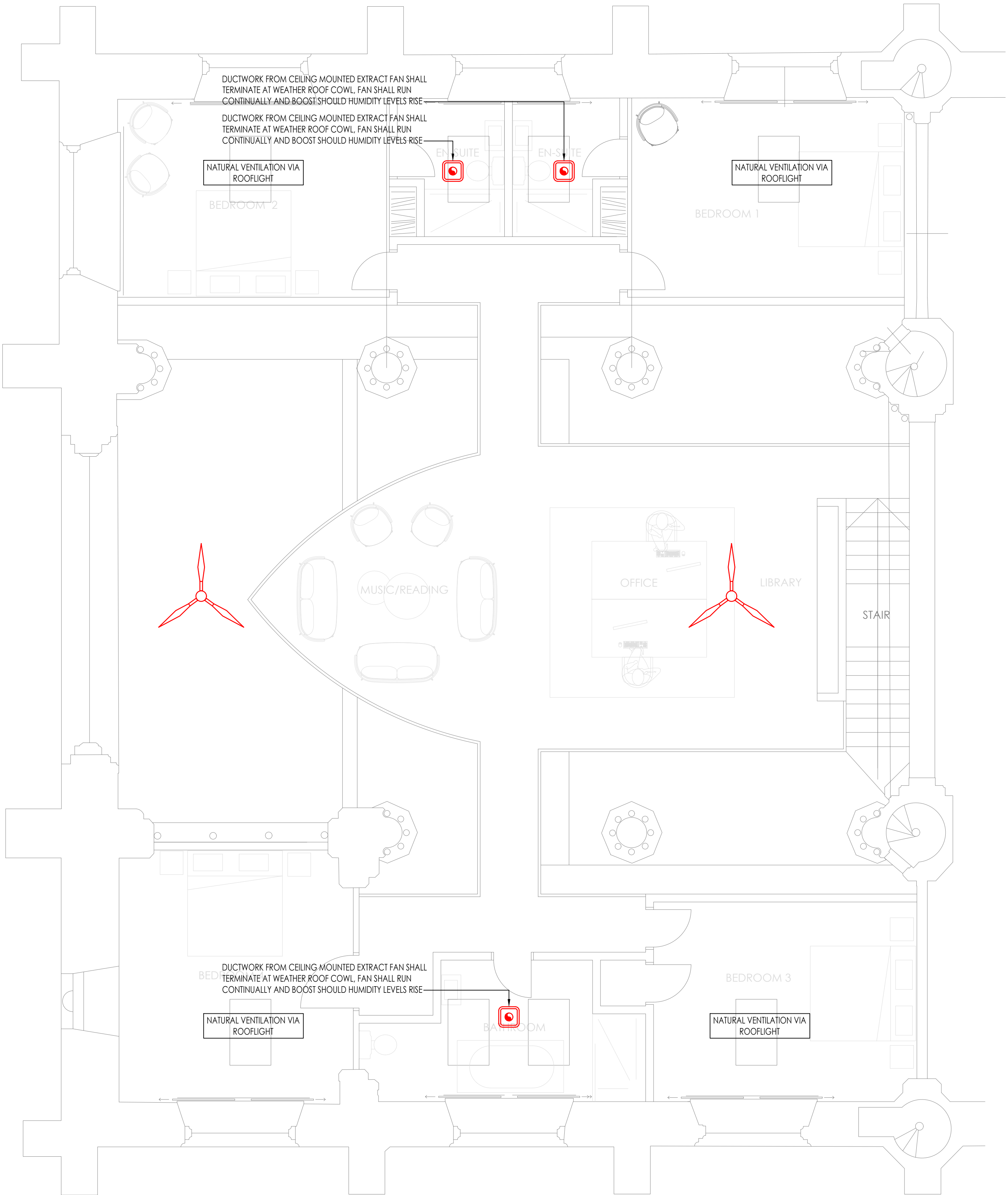
INDICATIVE VENTILATION STRATEGY, FIRST FLOOR SCALE 1:50 @A0
