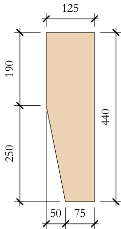
TcV_02 Elevation Left 1 : 10
