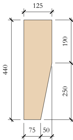
TcV_02 Elevation Left 1 : 10
