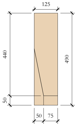
TcV_01 Elevation Left 1 : 10
