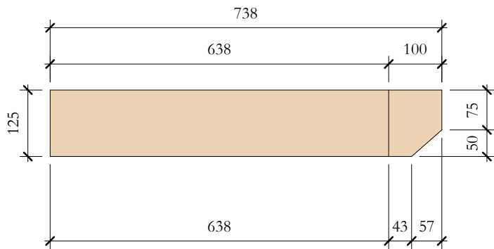
TcV_01 Elevation Top 1 : 10
