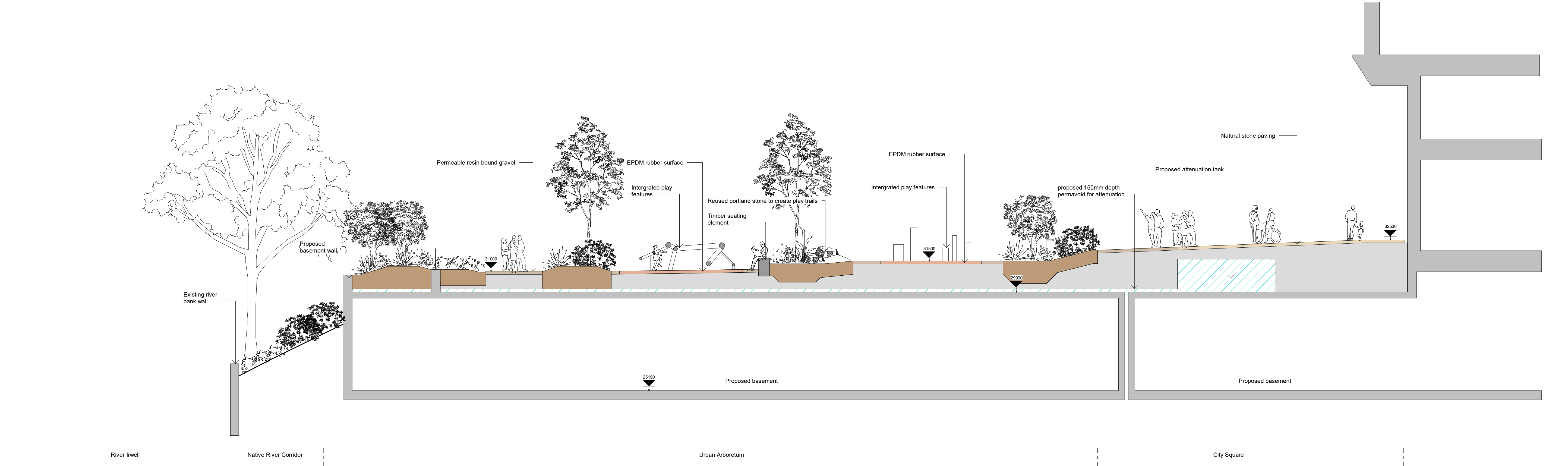
Section BB Scale 1:100
