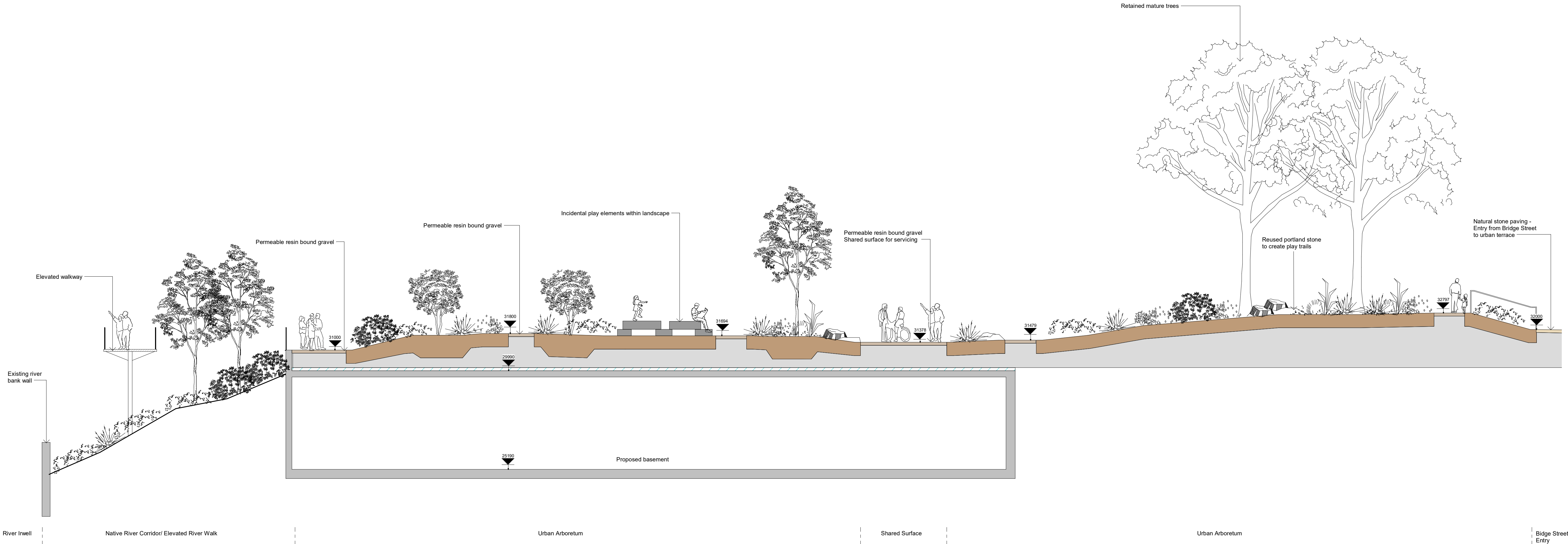
Section AA Scale 1:100
