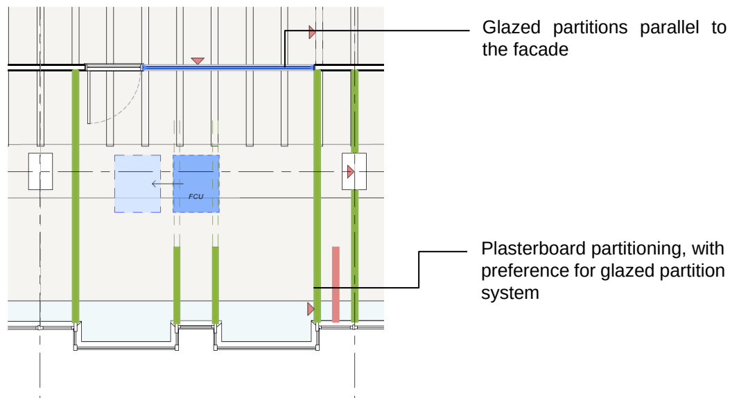
Fig. 07 – Glazed Partition Setout Parameters (Sketch provided by Sheppard Robson)
