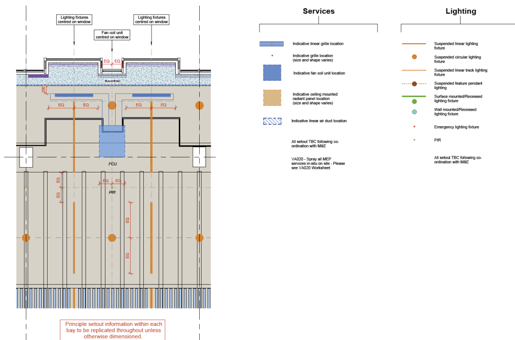
Fig. 12 – Lighting & MEP Setout Principles Sketch (Sketch provided by Sheppard Robson)
