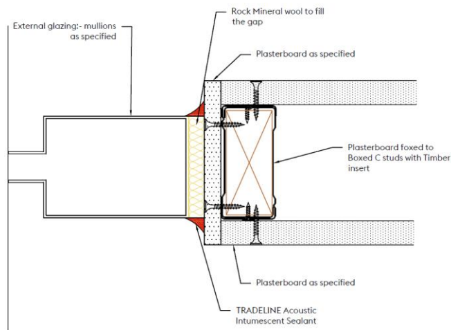
Fig. 04 – Partition Abutment to Heritage Curtain Wall Mullion Detail (Sketch provided by Topline Interiors and Tradeline)
