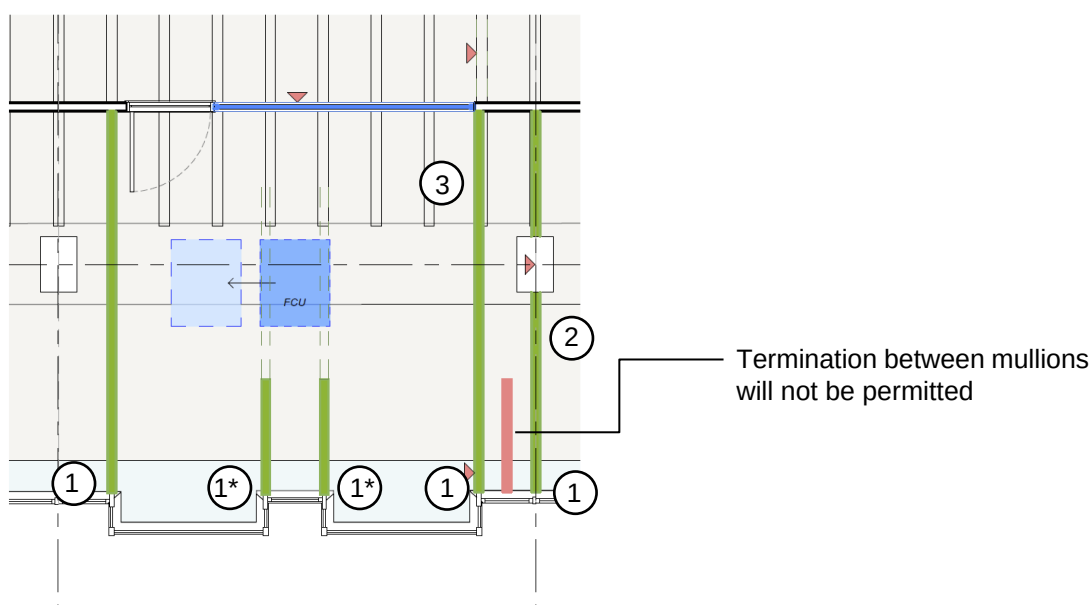
Fig 06. – Partition Setout Parameters (Sketch provided by Sheppard Robson)
