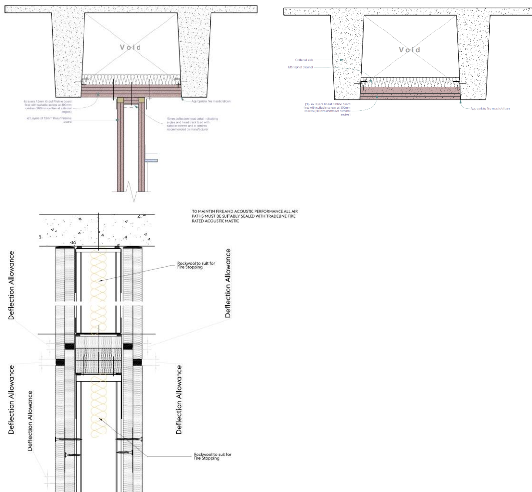
Fig 05. – Partition Head Details to Coffers (Sketches provided by Topline Interiors and Tradeline)
