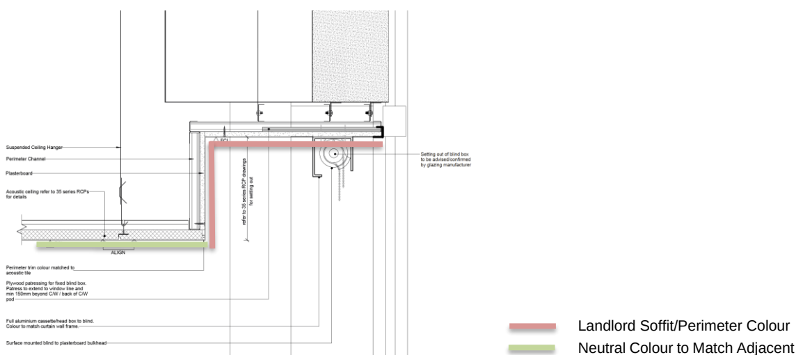
Fig. 10 – Perimeter Bulkhead Sketch (Sketch provided by Sheppard Robson)
