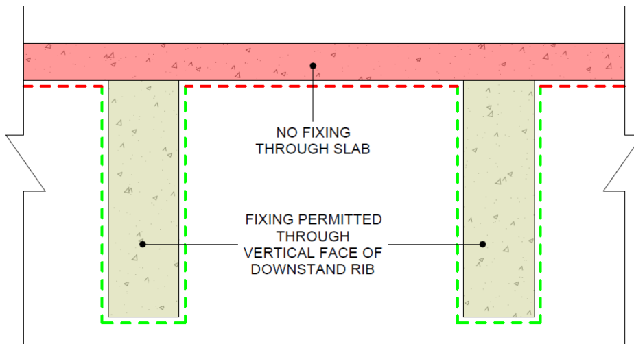
Fig. 03 – Section Diagram of Ribbed Slab Fixing Parameters (Sketch provided by Sheppard Robson)
