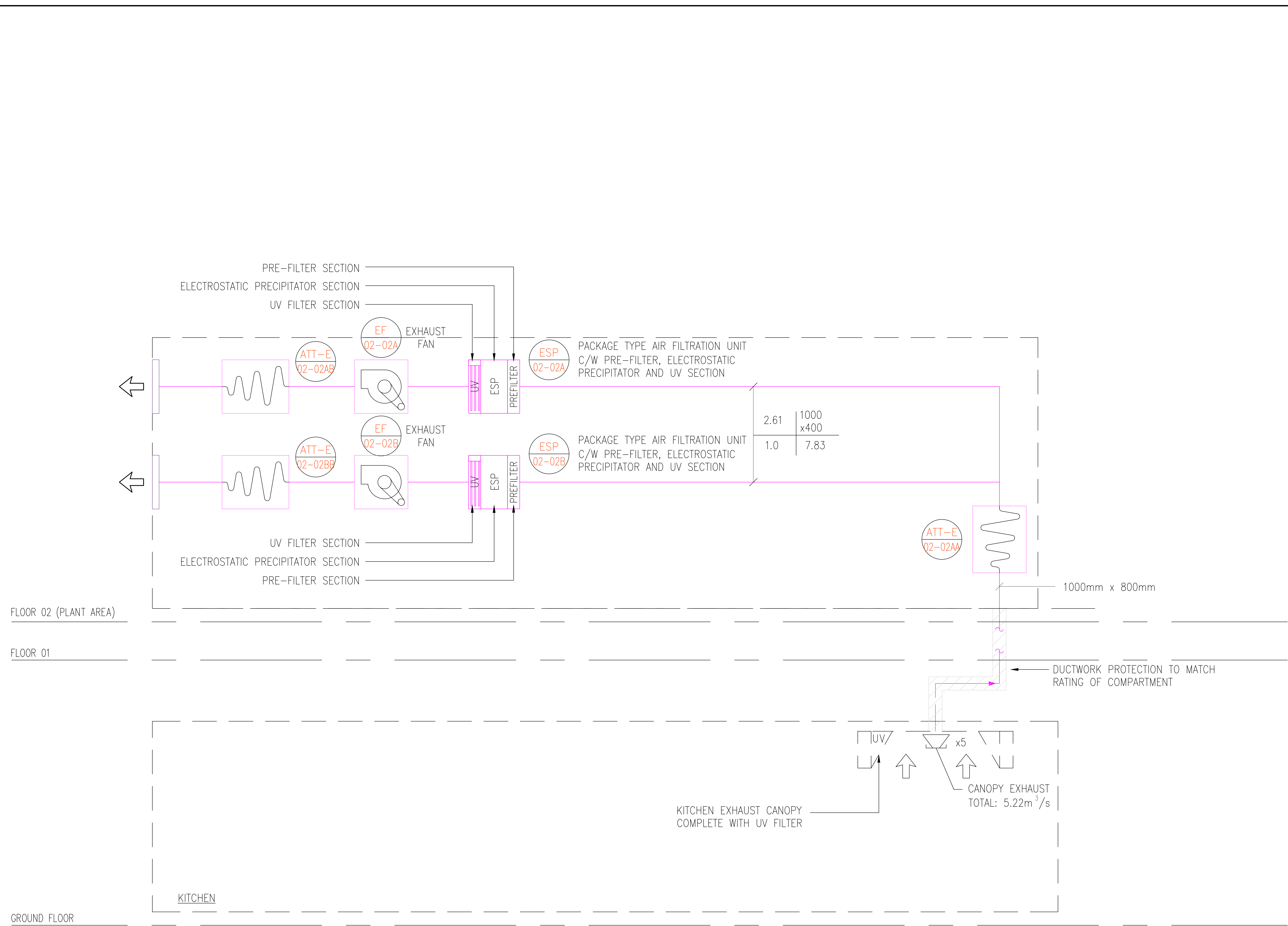
LEVEL00 KITCHEN EXTRACT SYSTEM SCHEMATIC
