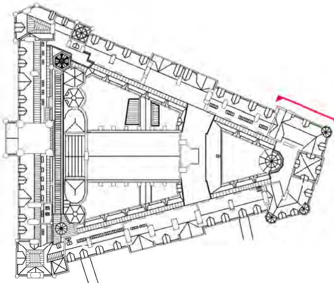
Key plan_Princess Street roof elevation 1 1 : 1250
