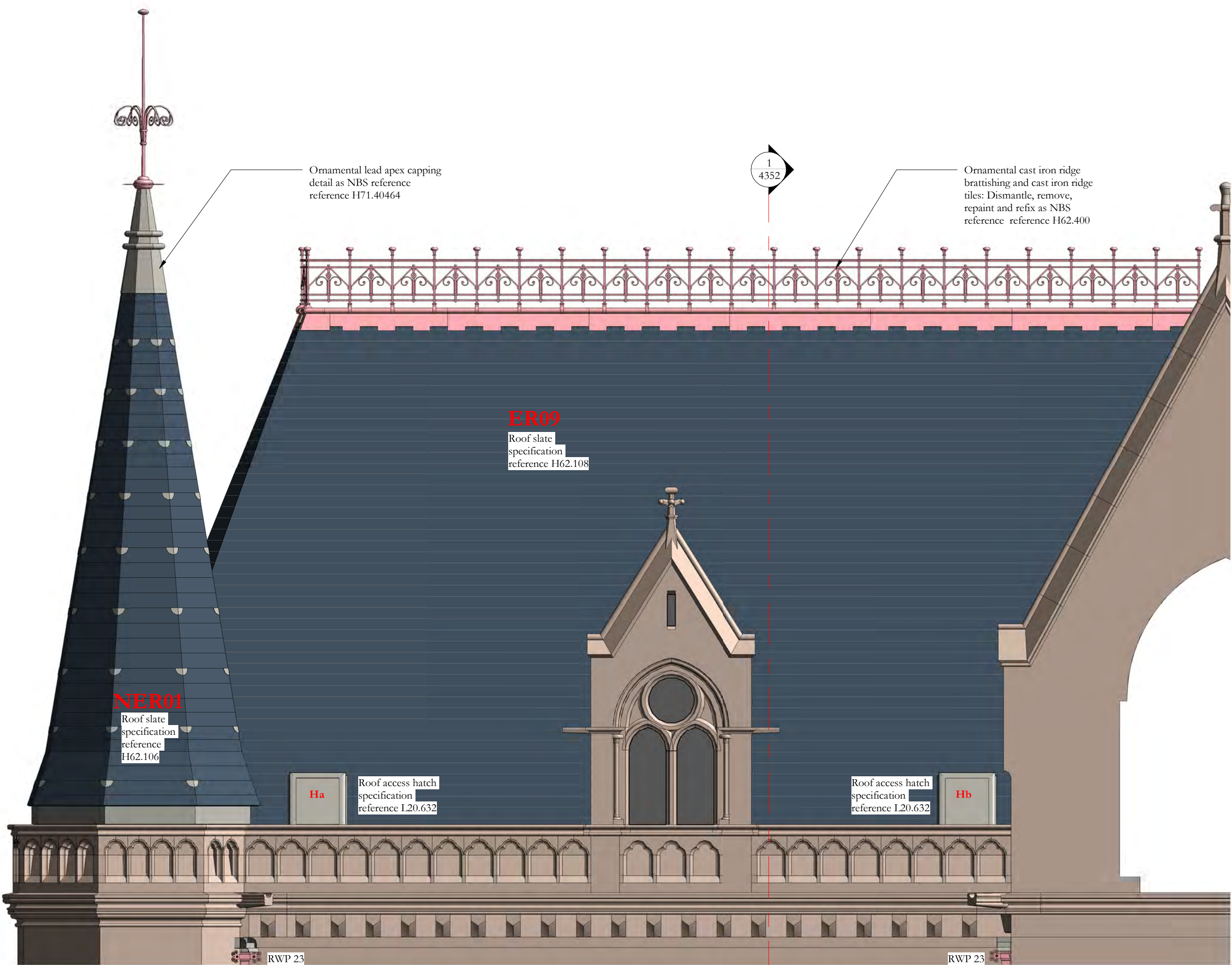
Princess Street roof elevation 1 1 : 50
