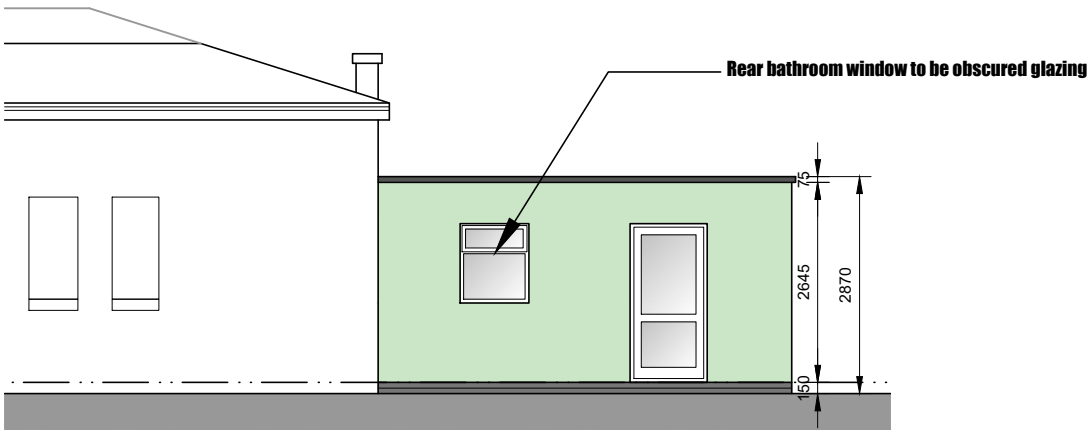
South Facing Rear Elevation
