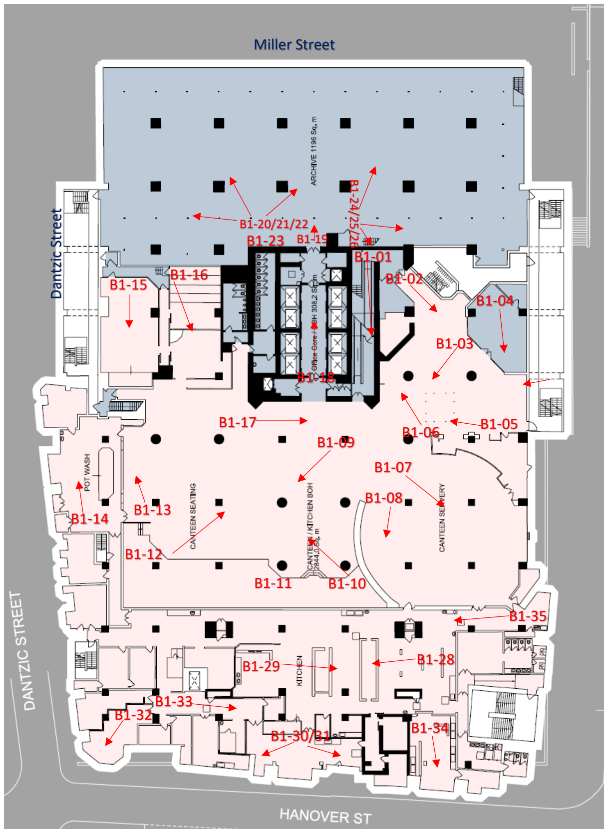
Figure 1. Location and direction of Level B1 views. Extract from Simpson Haugh drg.no.: 10246-SHP-Z1-B1-XP-A-G200-001
