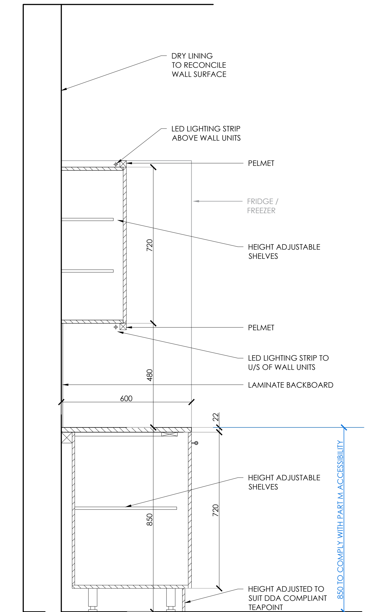
TYPICAL SECTION THROUGH TEAPOINT scale 1:10
