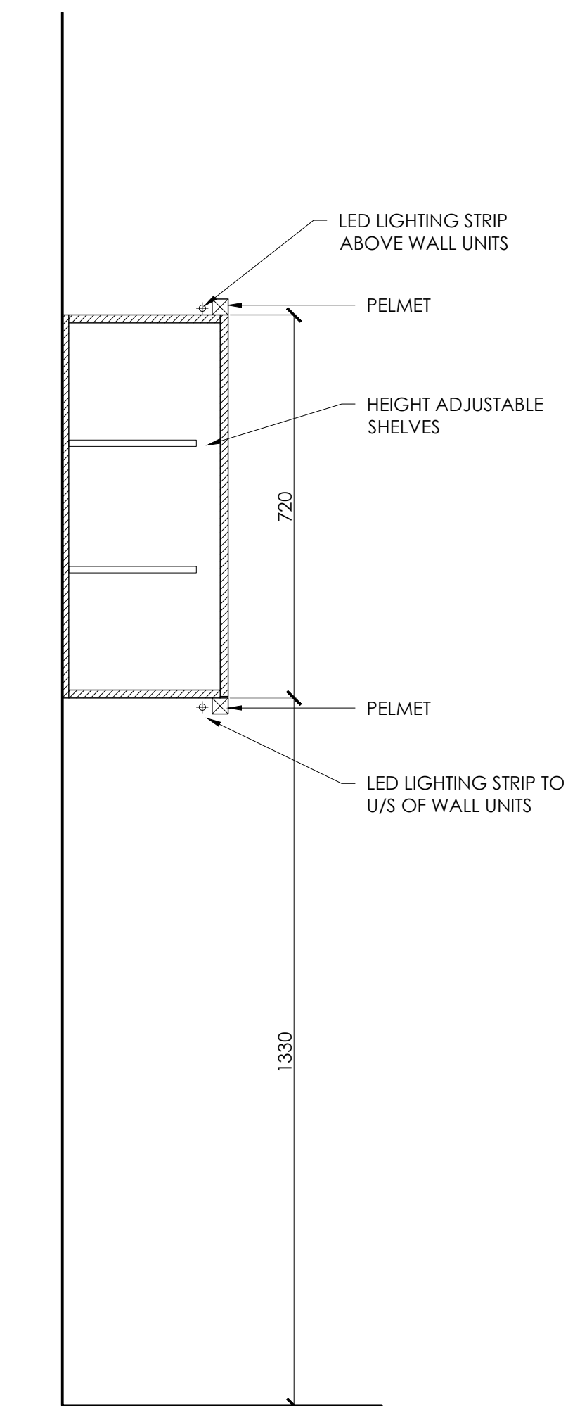
TYPICAL SECTION THROUGH PRINT POINT scale 1:10
