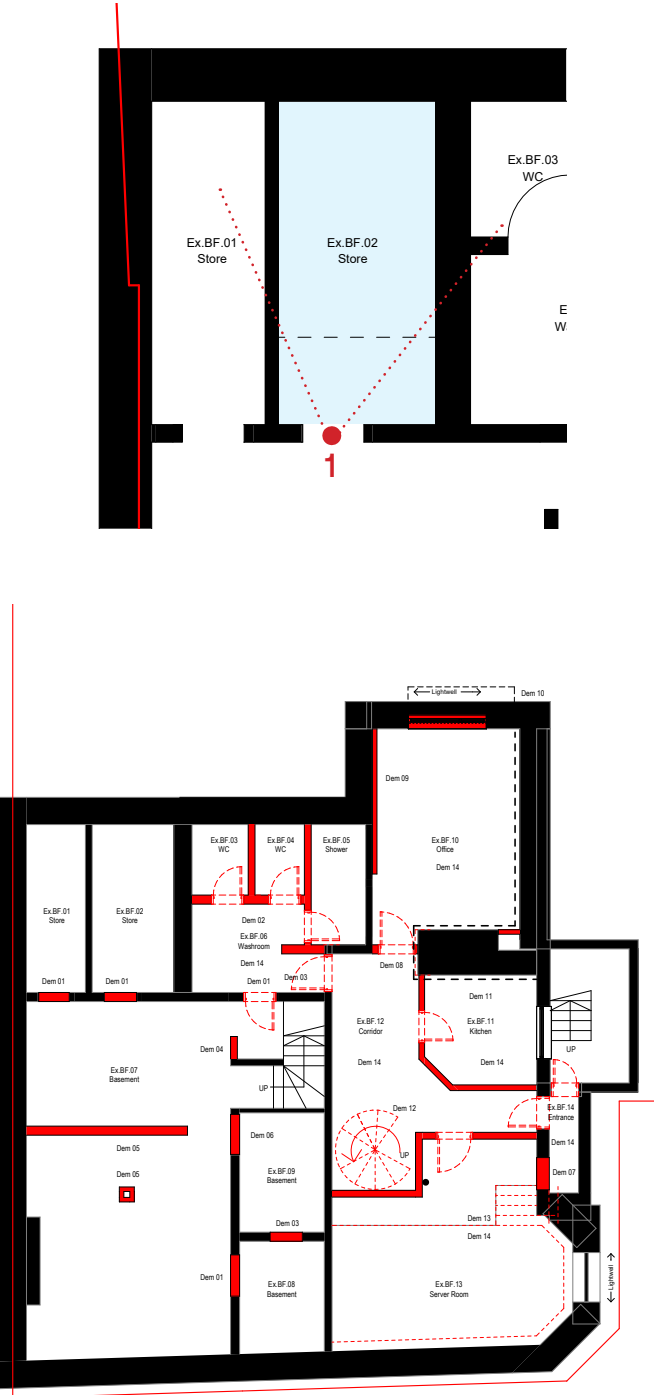
Basement Floor Demolition Plan
