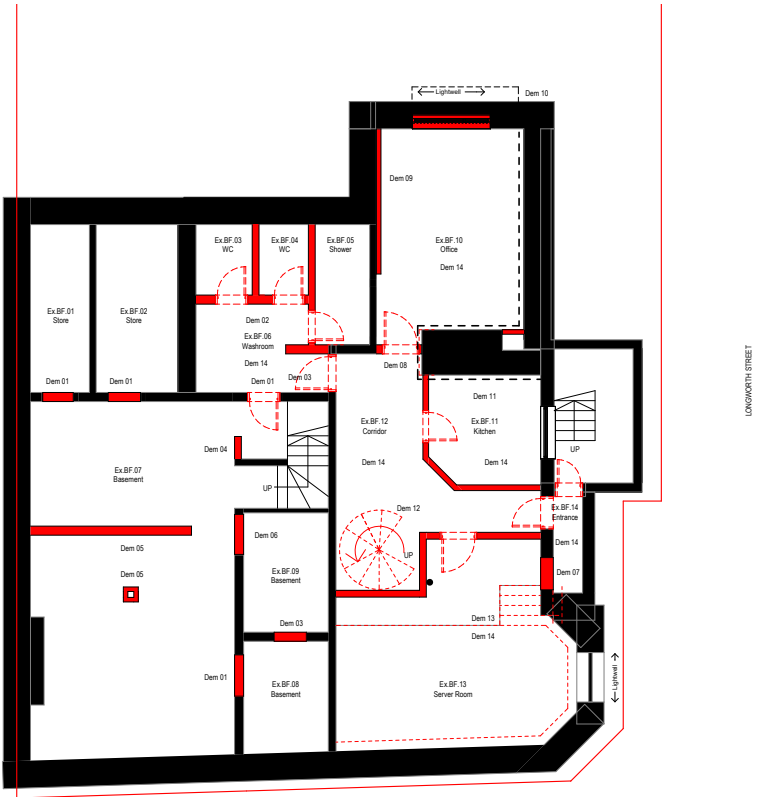
Basement Floor Demolition Plan
