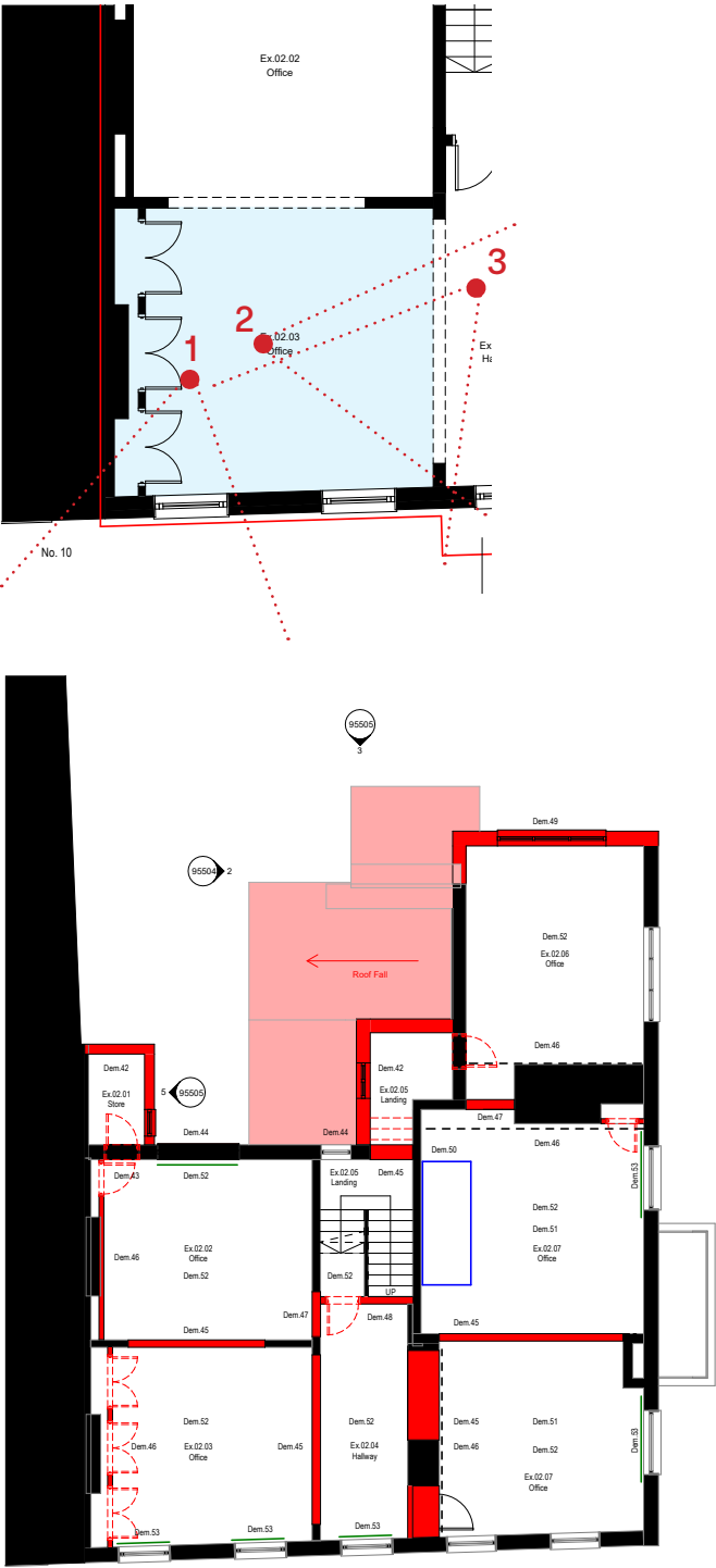
First Floor Demolition Plan
