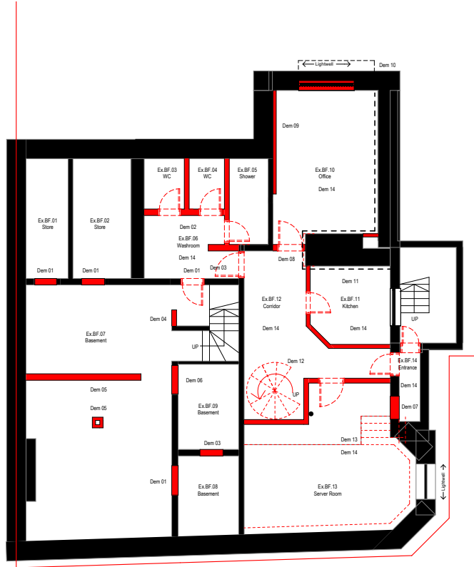
Basement Floor Demolition Plan
