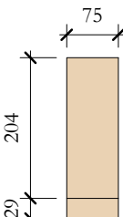
TcR_06 Elevation Left 1 : 10
