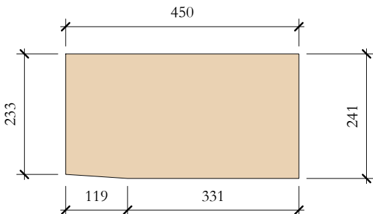
TcR_07 Elevation Front 1 : 10
