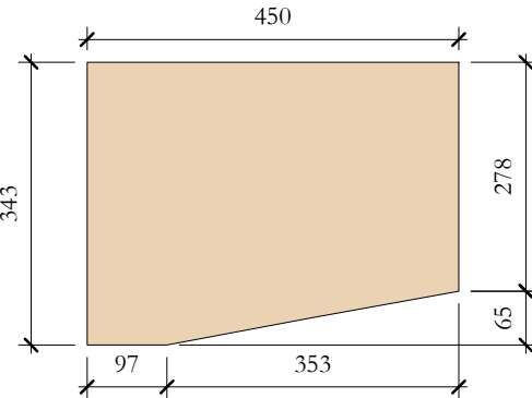
Elevation Front 1 : 10
