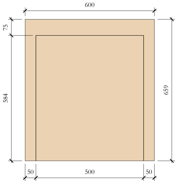
TcP_02 Elevation Front 1 : 10
