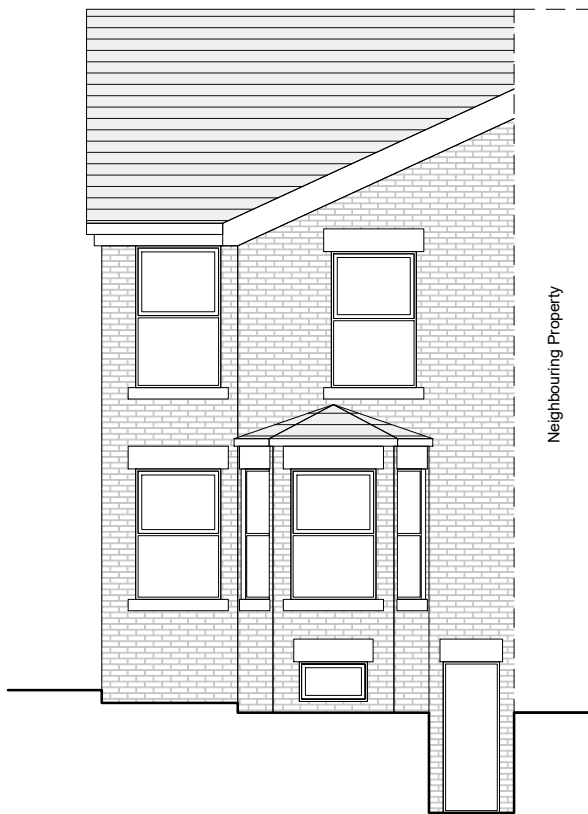
3 Rear Elevation 1 : 100
