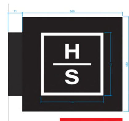
Front Elevation Scale 1:5 @ A3
