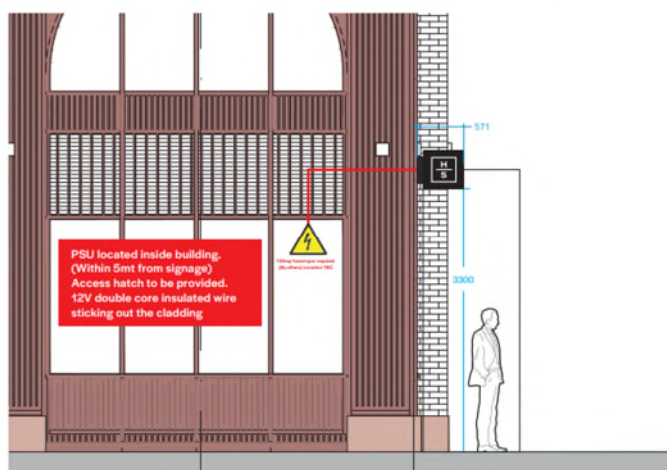
Setting Out - Facing East Elevation Scale 1:40 @ A3
