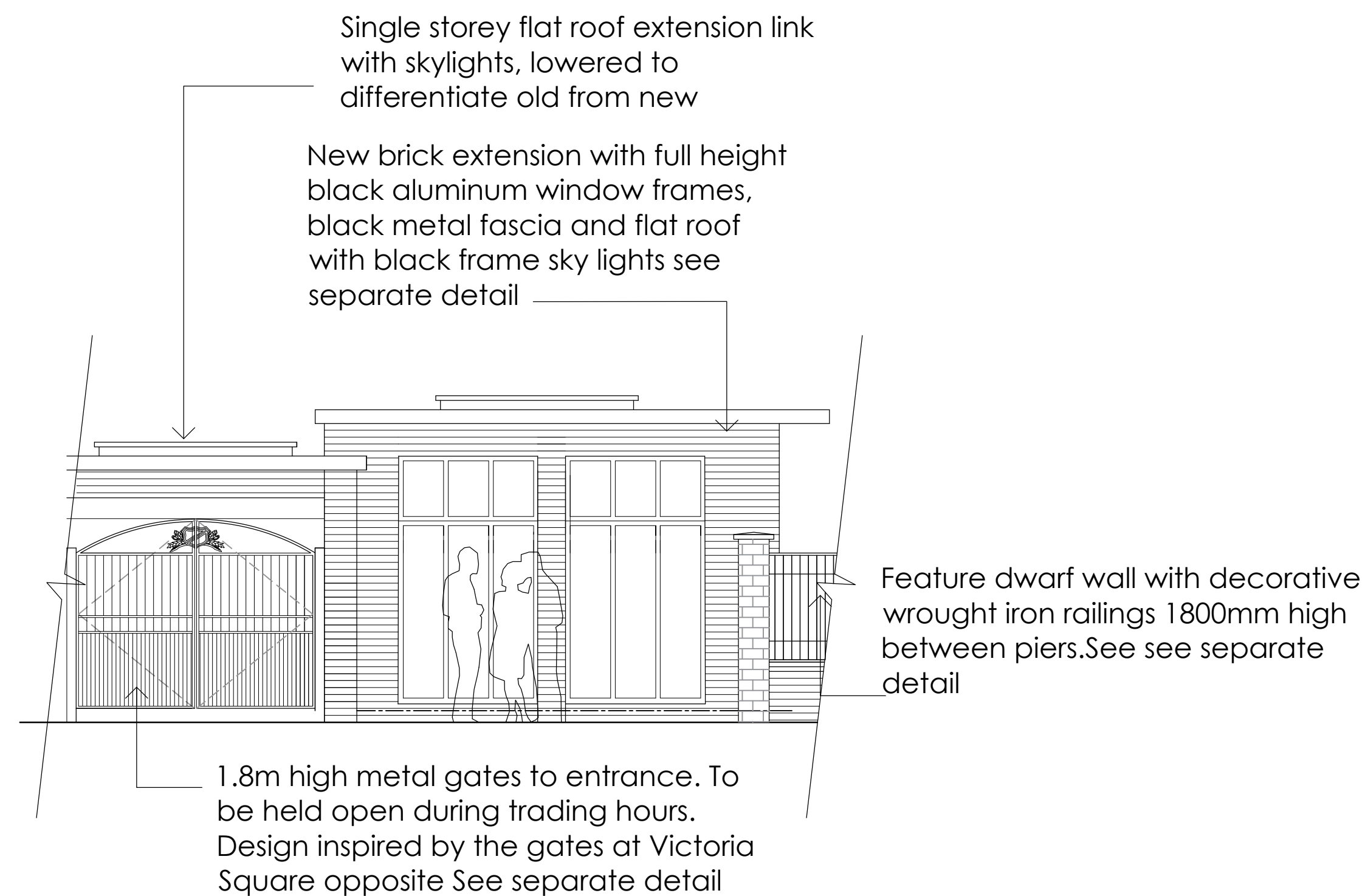
PROPOSED ELEVATION C - (BENGAL ST) Scale 1:50 @ A1 ,Behind boundary wall and railings.
