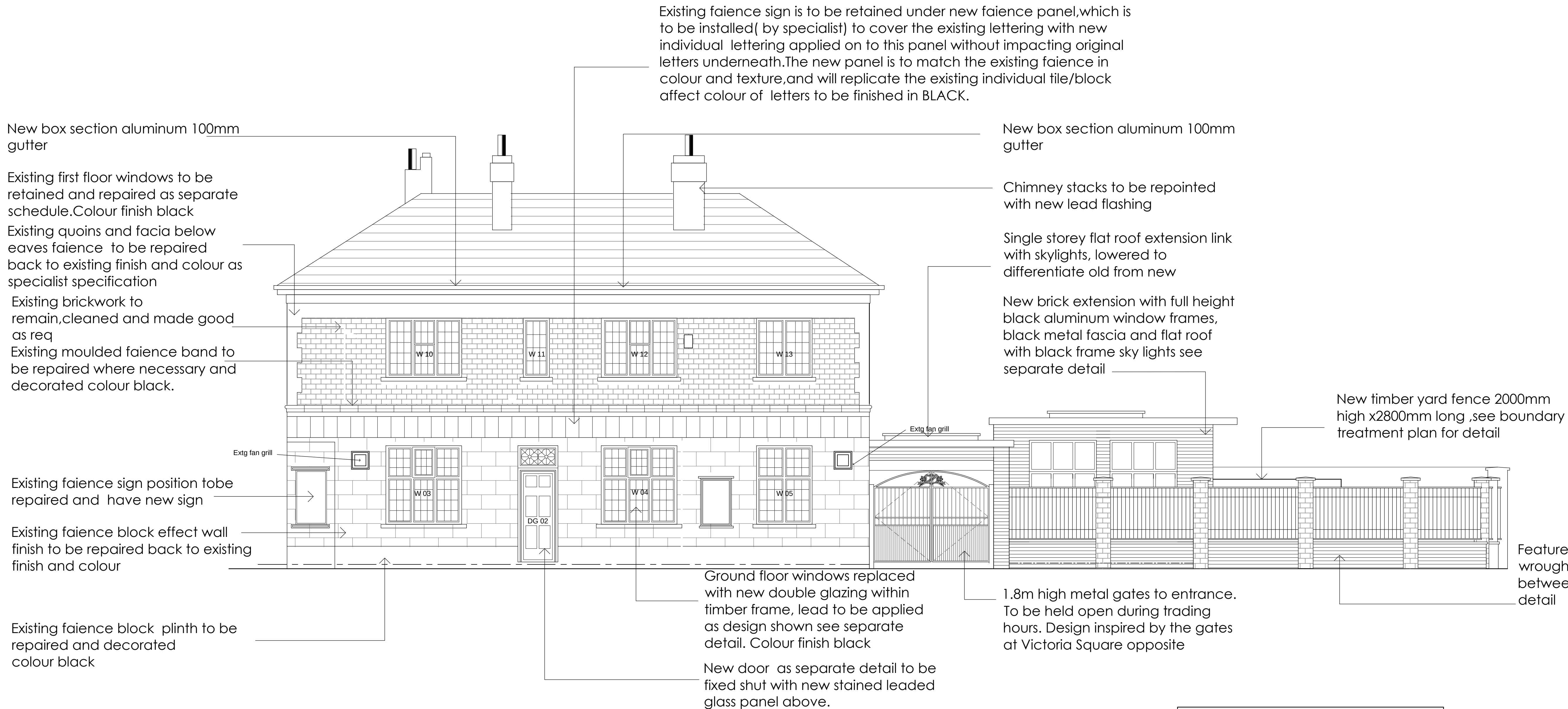
PROPOSED ELEVATION C - (BENGAL ST) Scale 1:50 @ A1
