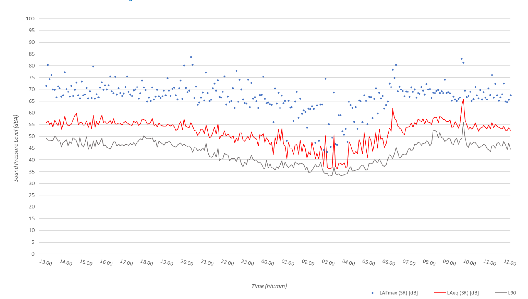
Figure 5: Measured Background Sound Levels Time History (M1): 14 th – 15 th May 2025
