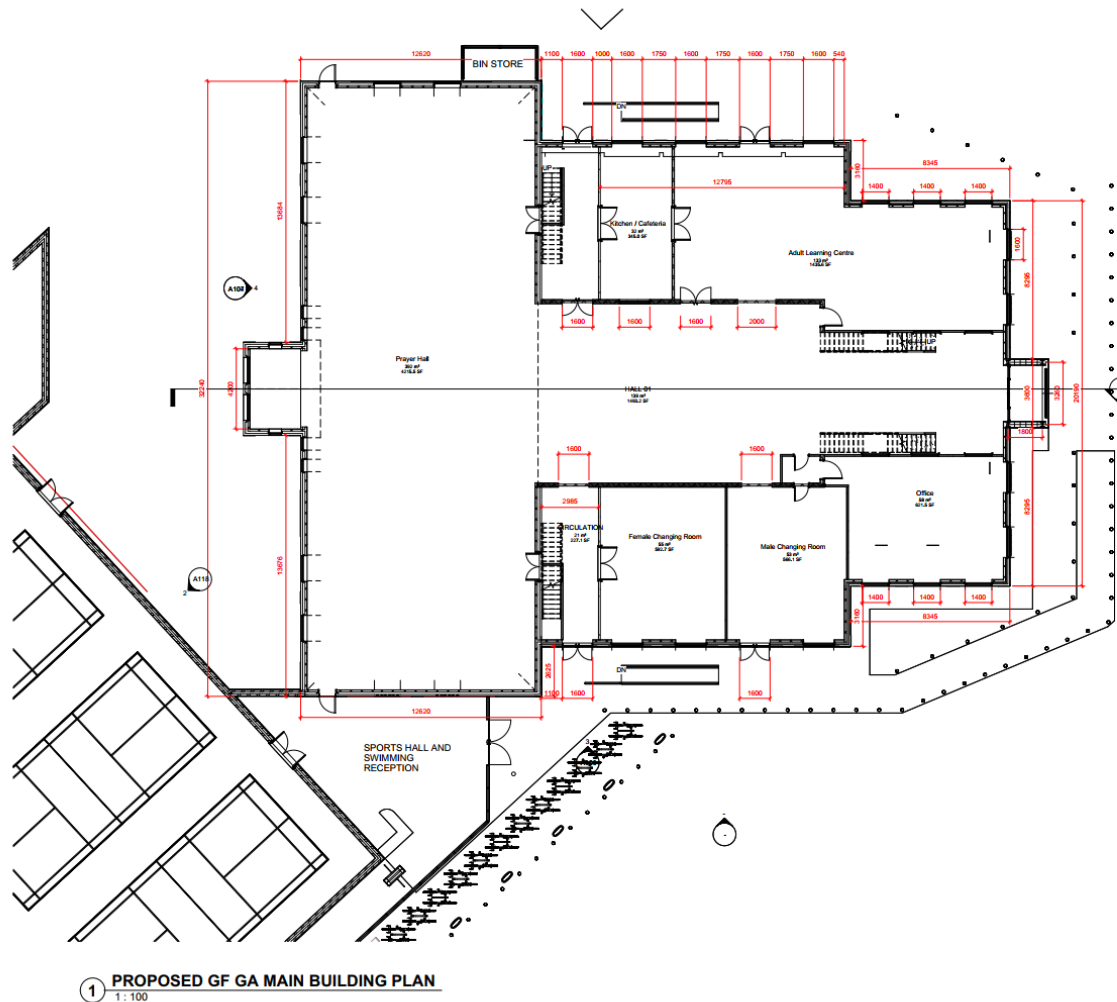
Figure 6: Site Plans Provided by 'NK Architectural'
