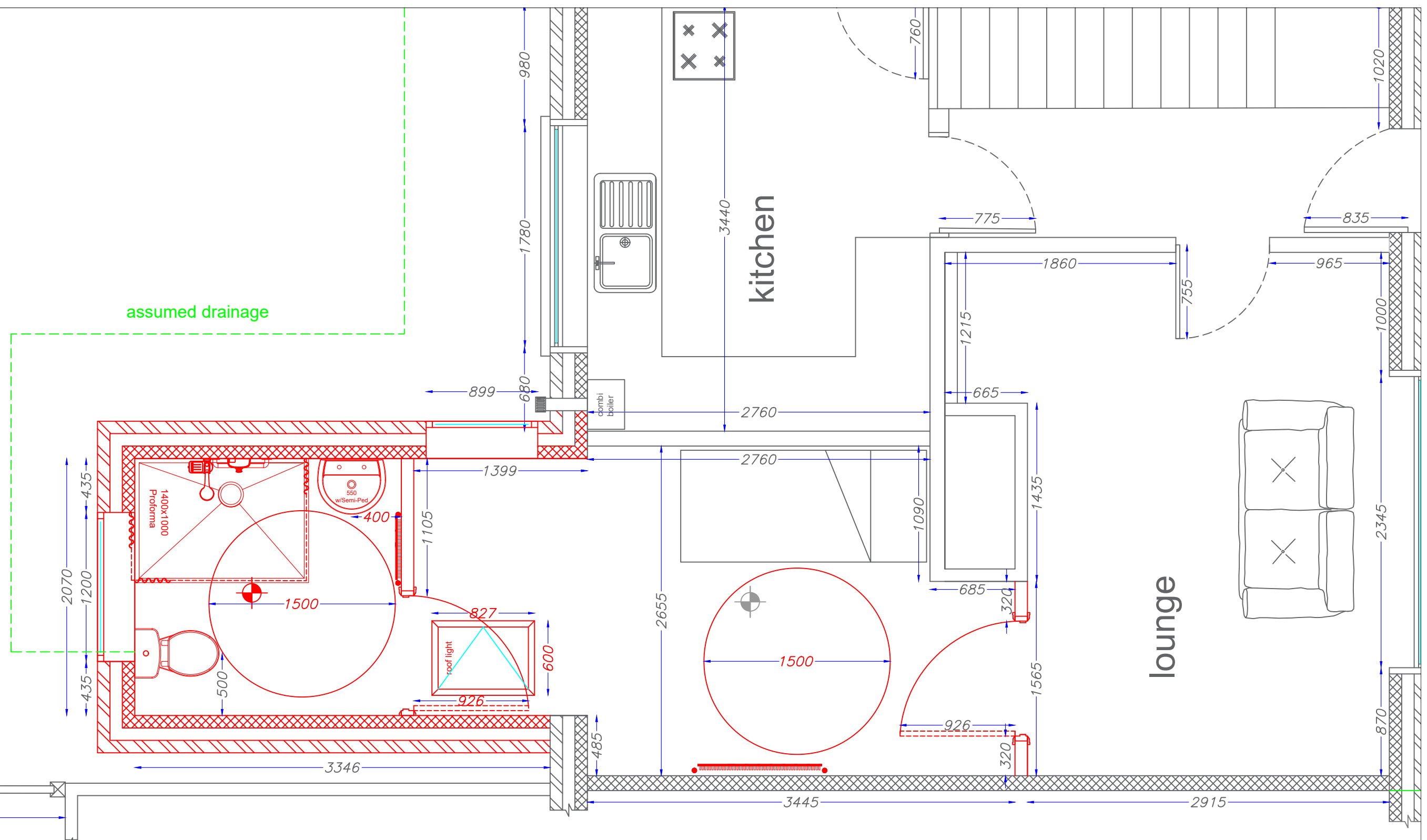
Proposed Layout
