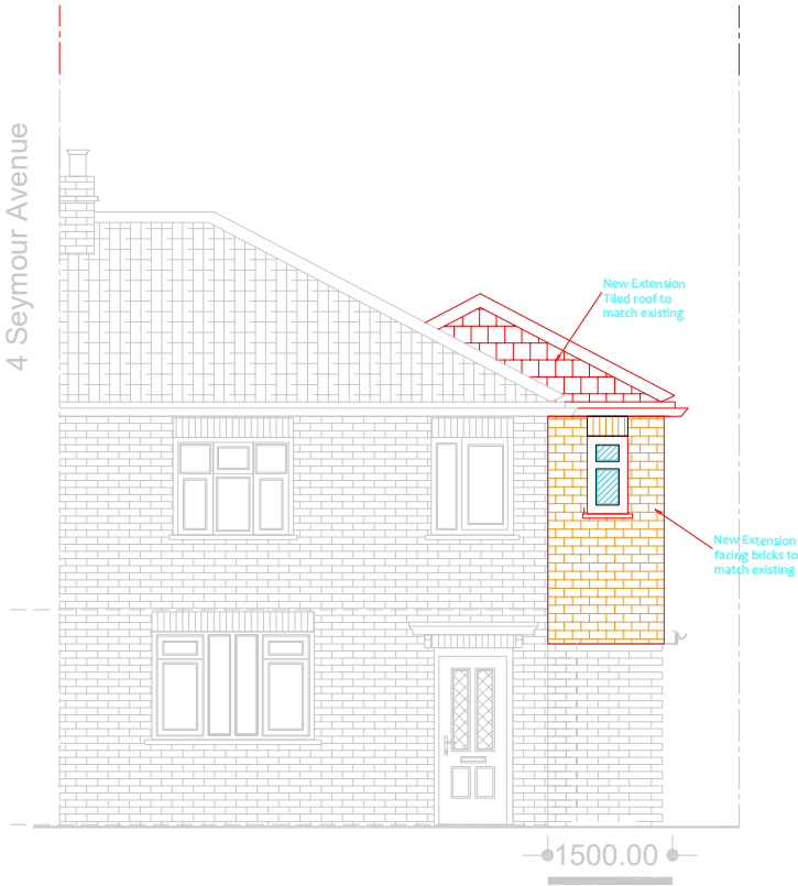
11 Proposed Front Elevation
