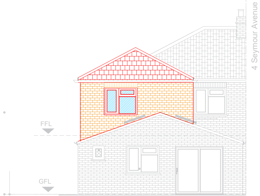
12 Proposed Rear Elevation
