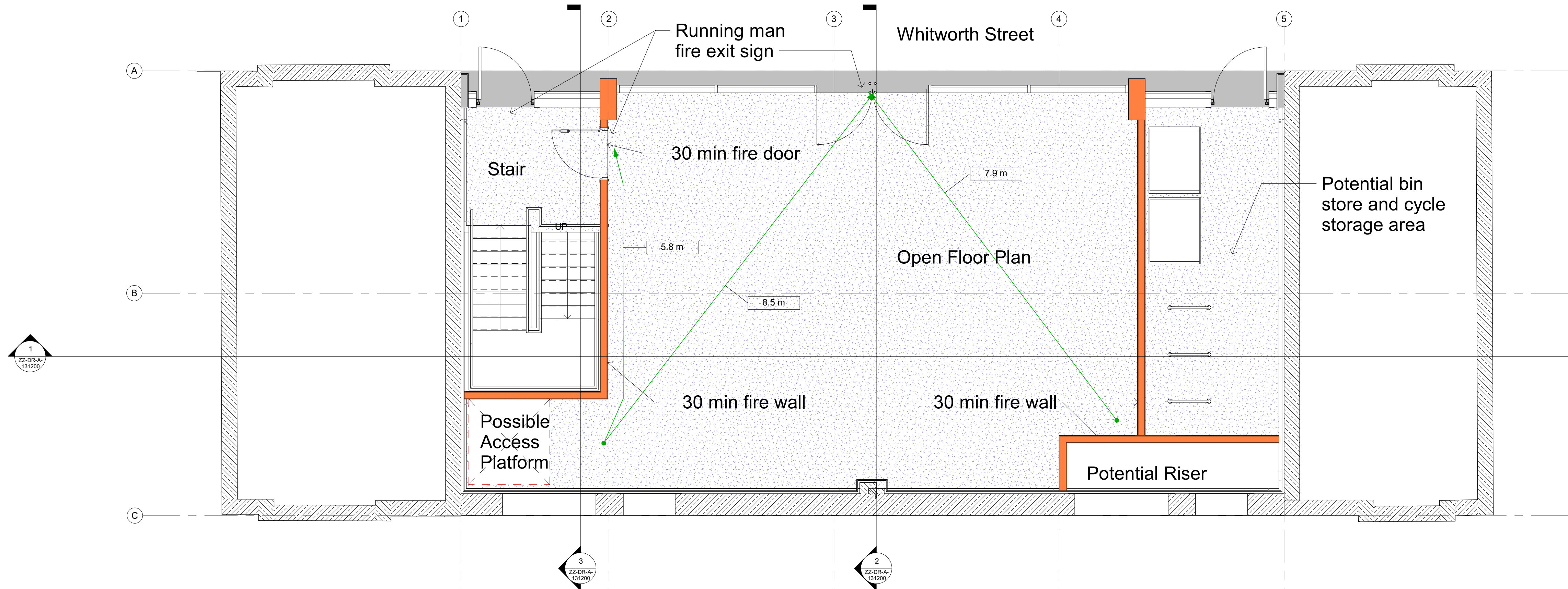
2 ZZ-DR-A- 131200 Planning Upper Ground Floor Fire Plan Scale: 1 : 50
