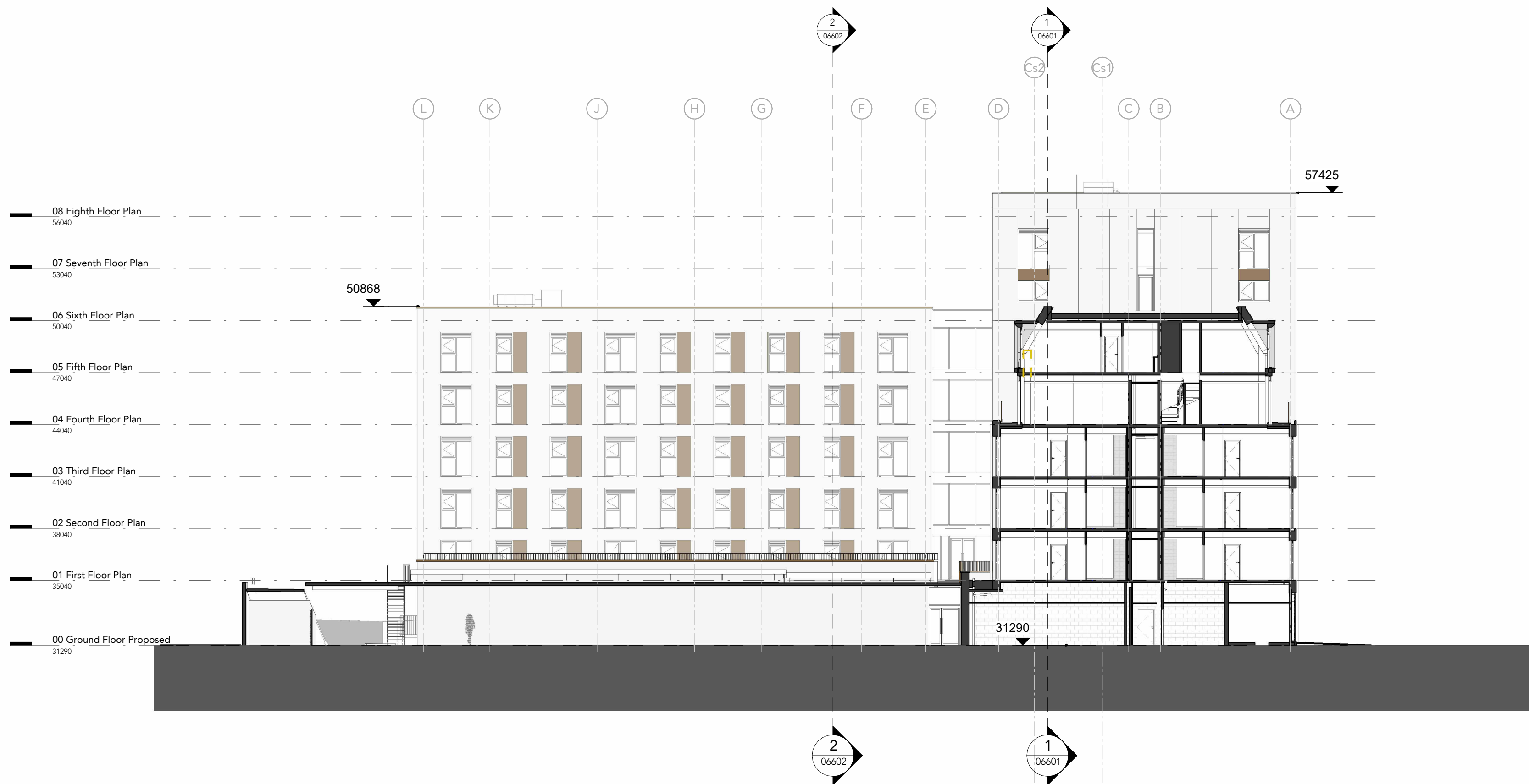
1 Section CC 1:200
