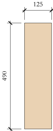
TcV_04 Elevation Left 1 : 10
