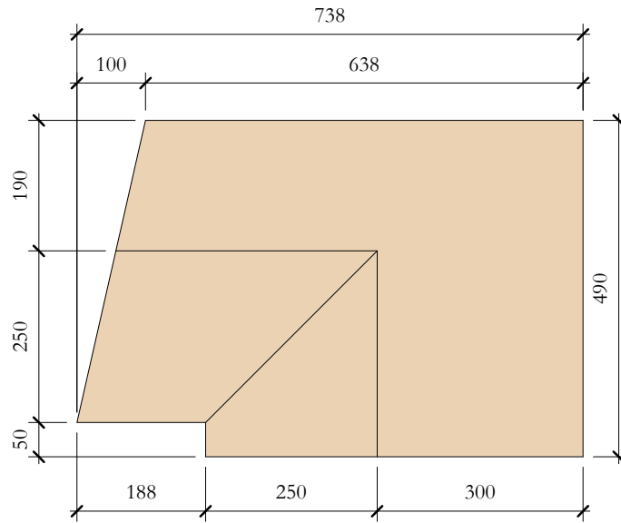
TcV_04 Elevation Front 1 : 10
