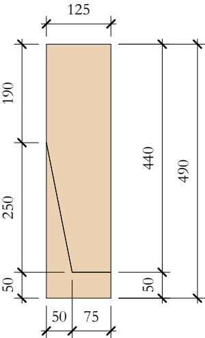
TcV_03 Elevation Left 1 : 10
