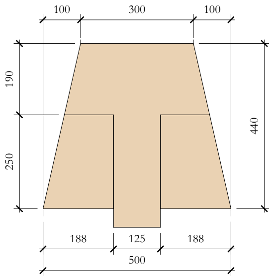
TcV_03 Elevation Front 1 : 10
