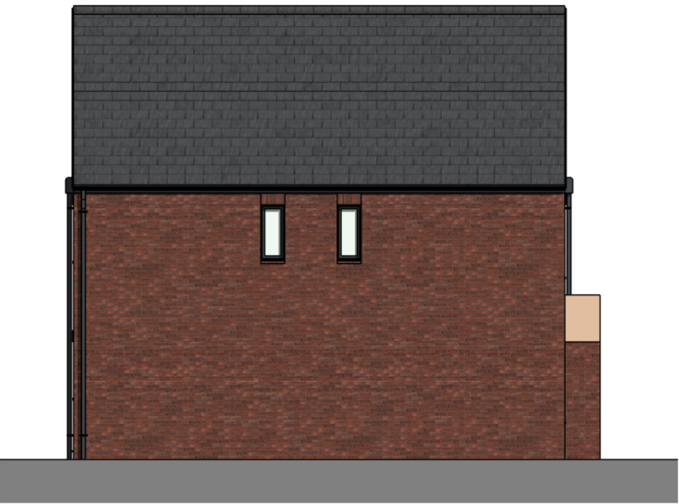
Left Elevation 1 : 100
