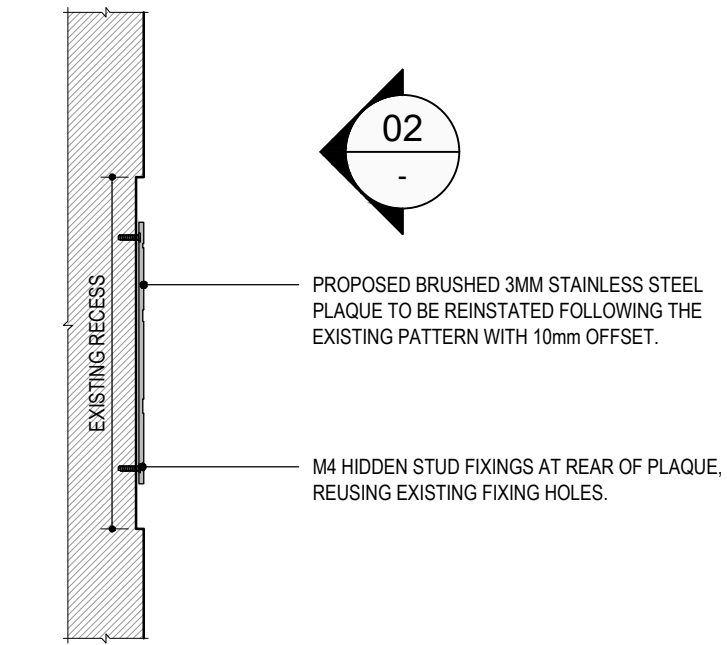
03 PROPOSED EXTERNAL PLAQUE SECTION DETAIL SCALE 1:5@A1; 1:10@A3
