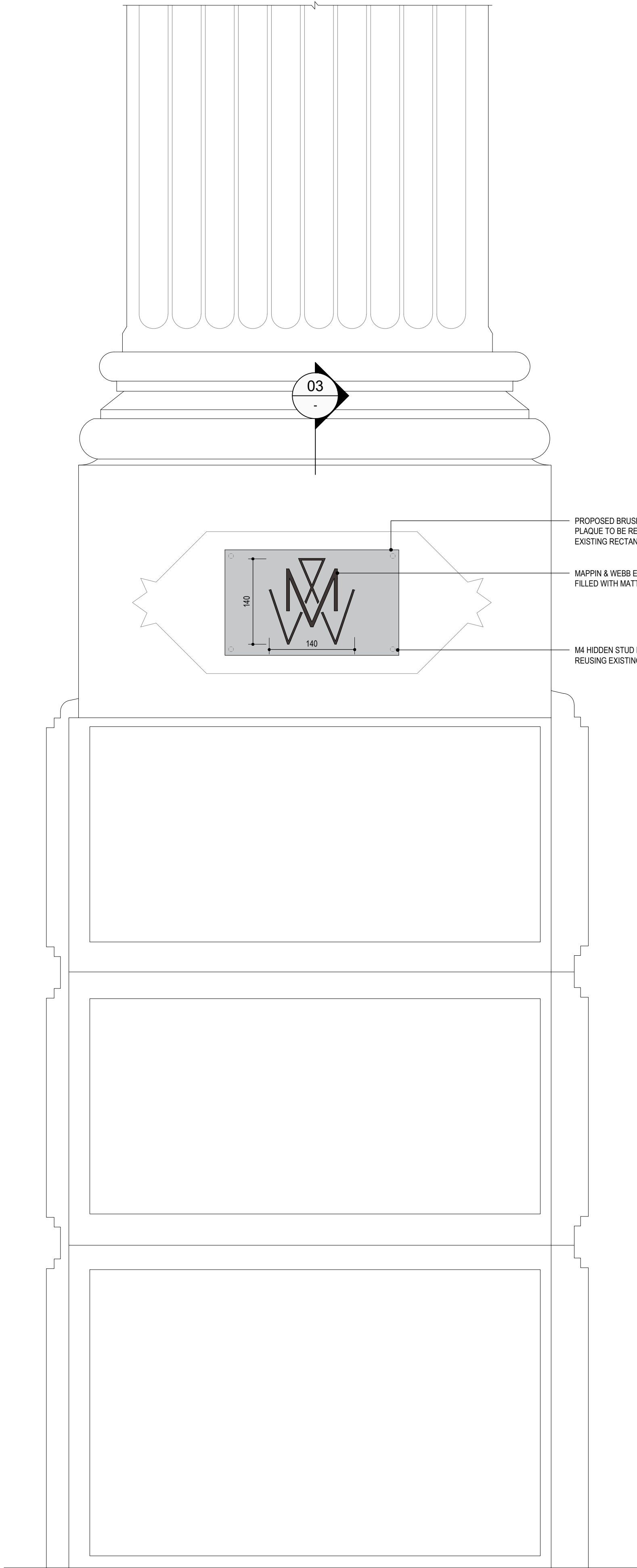
02 PROPOSED EXTERNAL PLAQUES SCALE 1:5@A1; 1:10@A3
