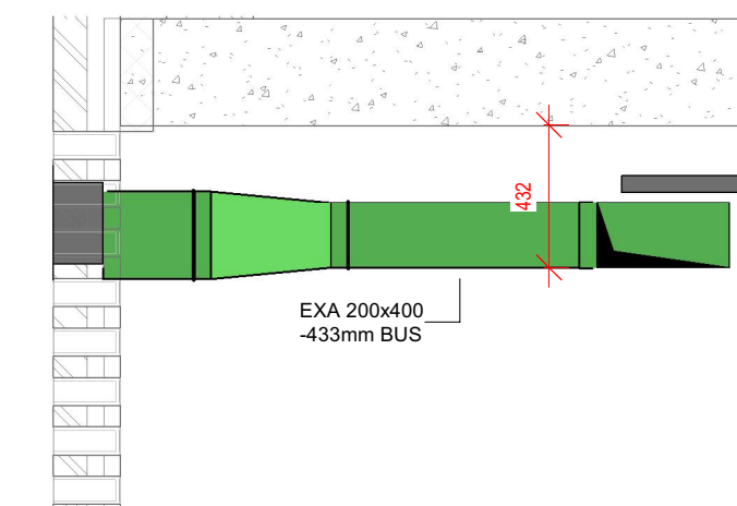
H Louvre Detail 1 1:25
