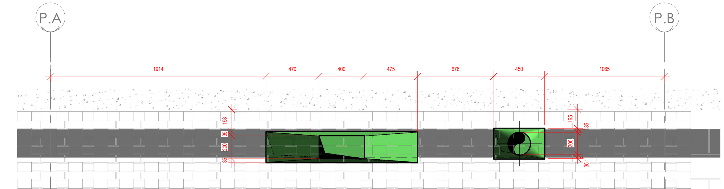
J Louvre Detail 3 1:20
