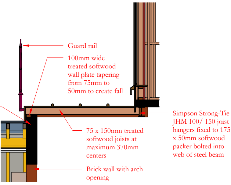
Section E-E
