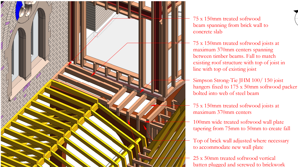
Isometric view
