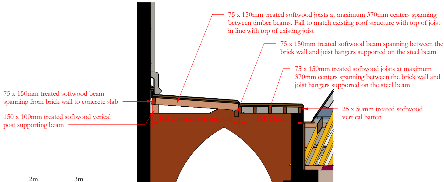
Section F-F
