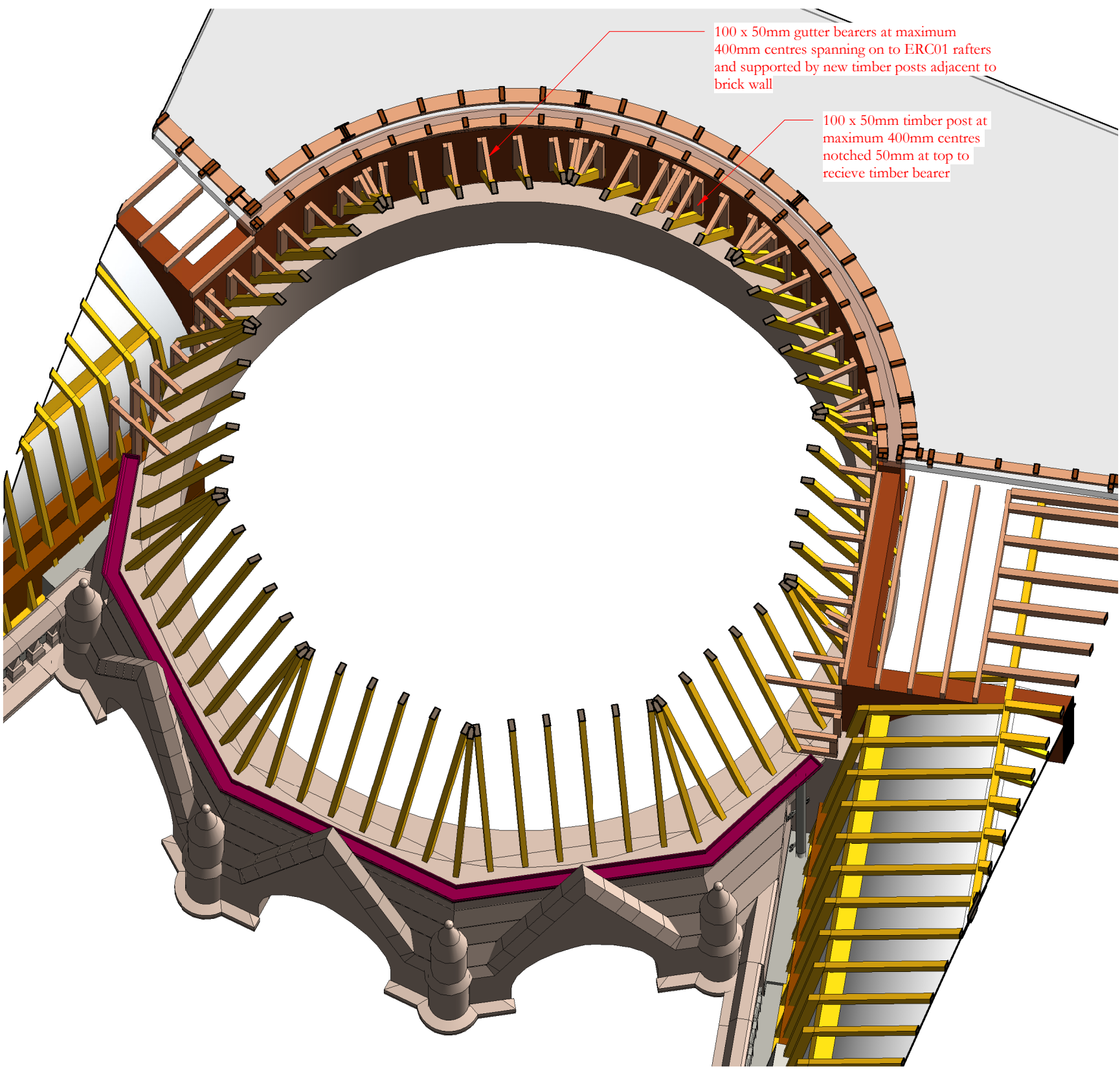
Isometric view showing gutter framing
