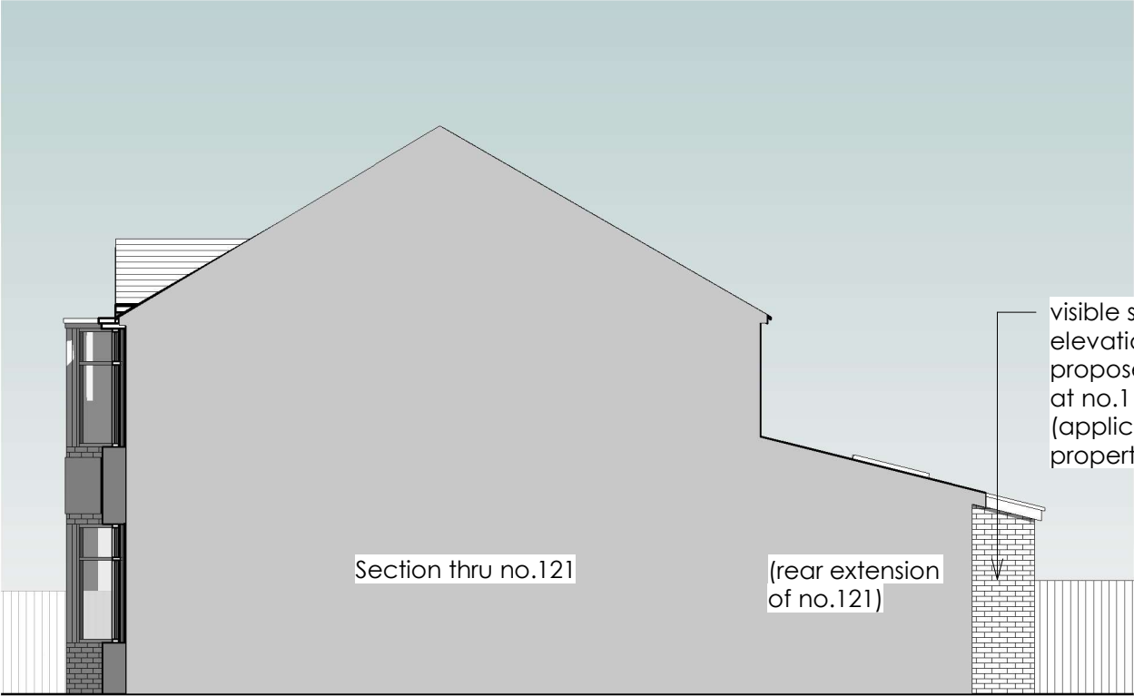
Proposed Side Elevation 02 @1:100
