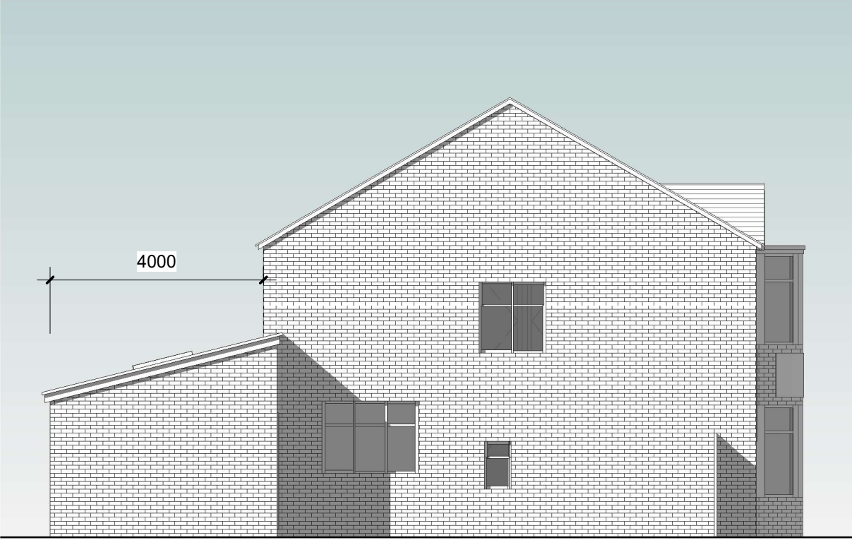
Proposed Side Elevation 01 @1:100
