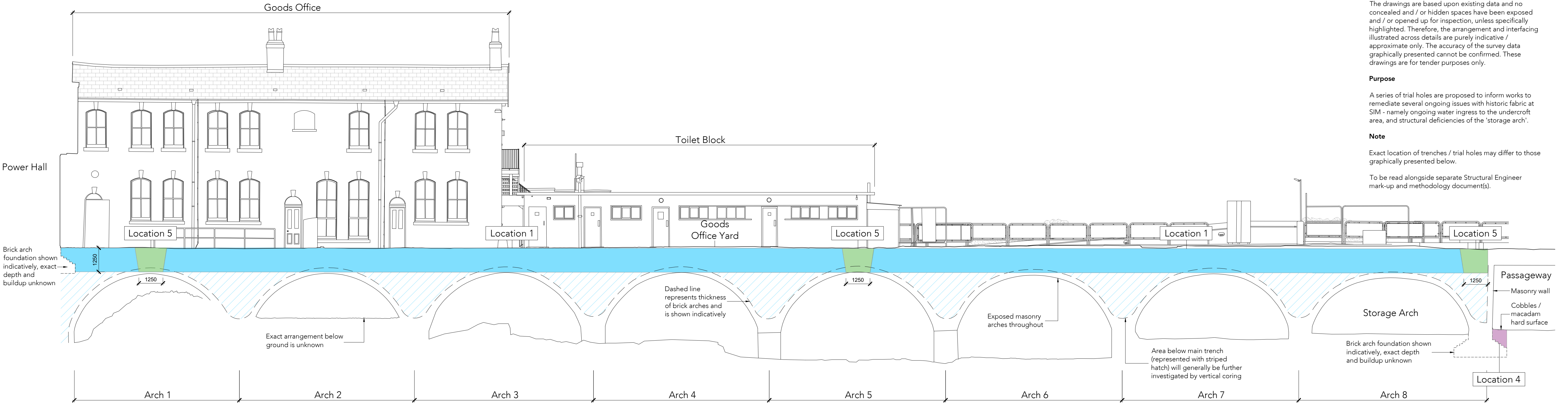
Goods Office Yard Section B-B as Existing - Proposed Trench Locations Scale 1:100
