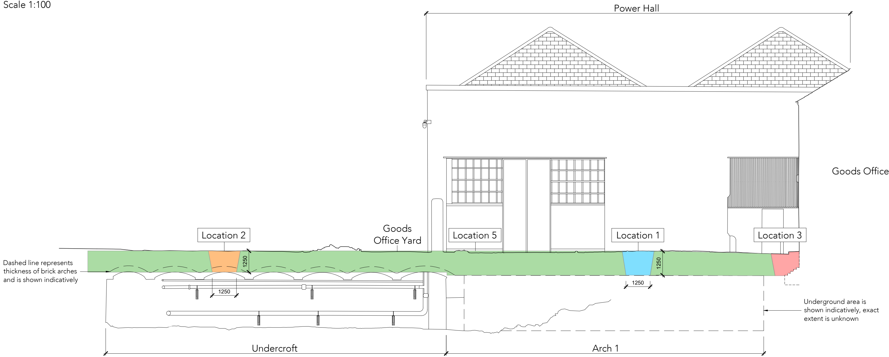
Goods Office Yard Section G-G as Existing - Proposed Trench Locations Scale 1:100
