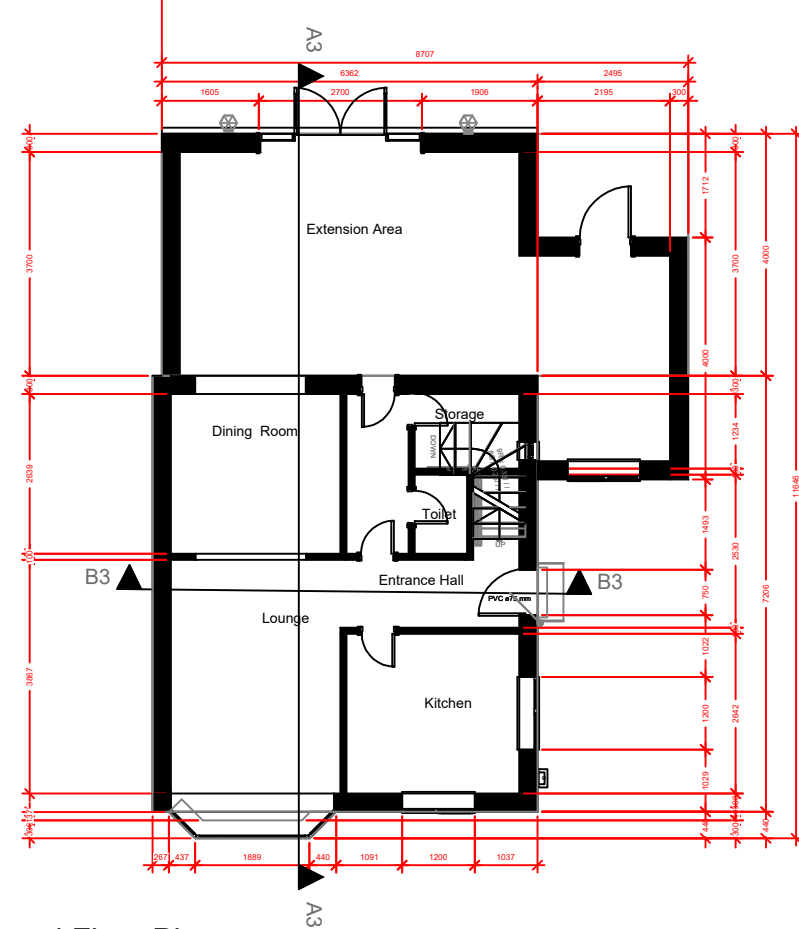
2 Prop Ground Floor Plan Scale 1:125@A3
